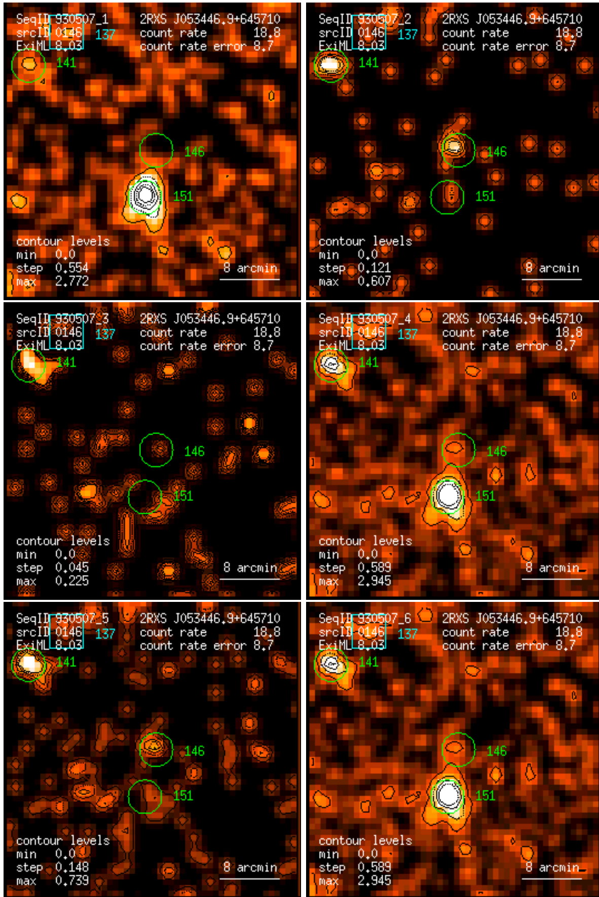
Figure 146: RASS 930507: detection 0146: band rate images, Gaussian filter: (1) PSPC channels 11 – 41, (2) 52 – 90, (3) 91 – 201, (4) 11 – 235, (5) 52 – 201, (6) 11 – 201. Broad band rates in counts/ks. Band rate contour levels in counts/ks/arcmin 2 .
