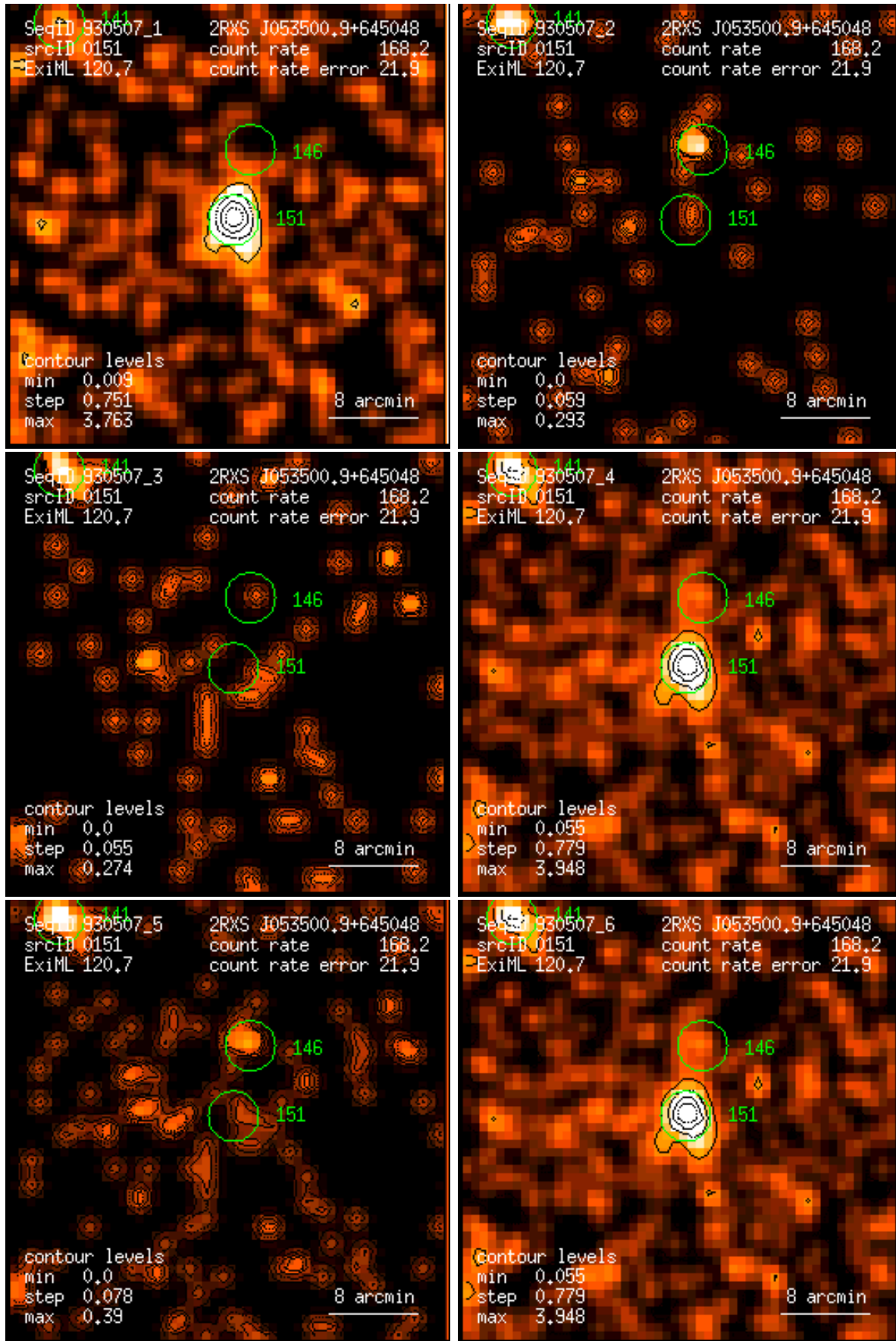
Figure 151: RASS 930507: detection 0151: band rate images, Gaussian filter: (1) PSPC channels 11 – 41, (2) 52 – 90, (3) 91 – 201, (4) 11 – 235, (5) 52 – 201, (6) 11 – 201. Broad band rates in counts/ks. Band rate contour levels in counts/ks/arcmin 2 .
