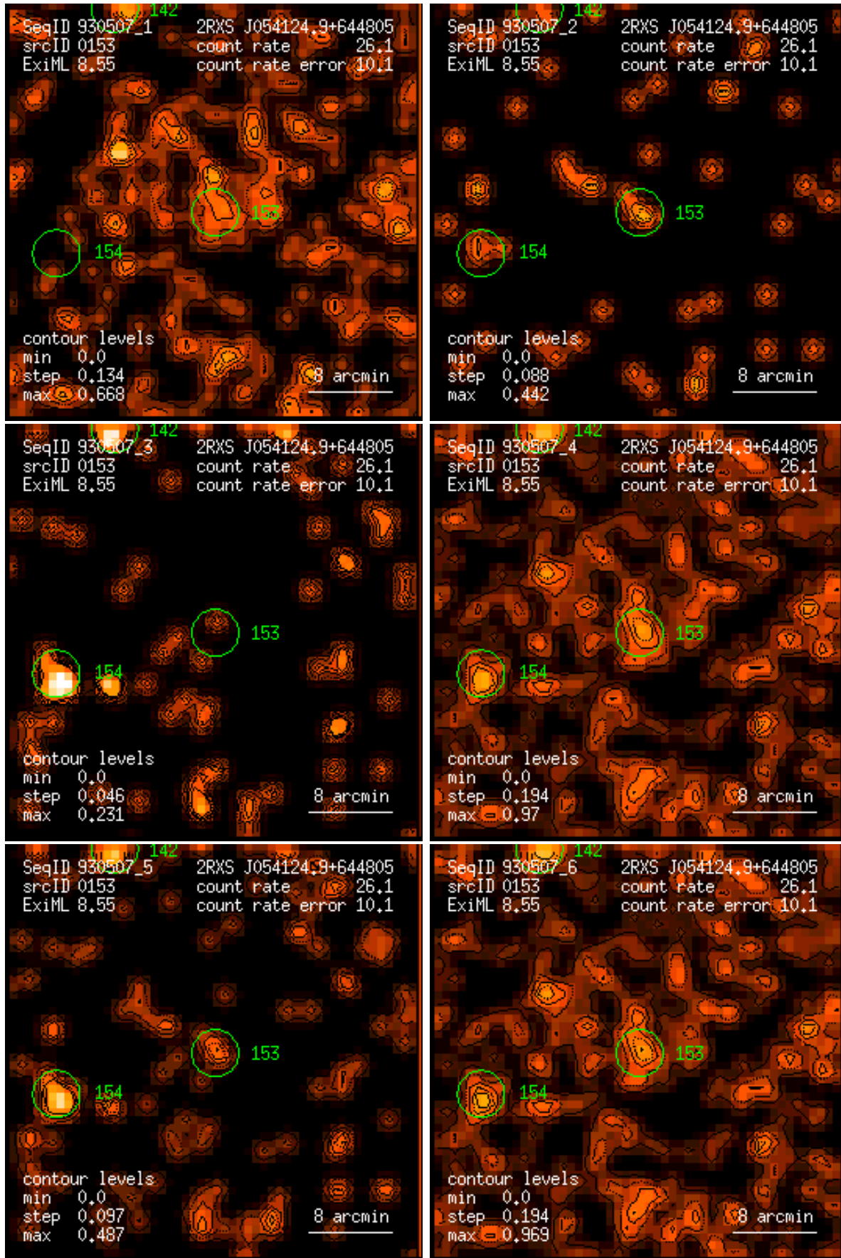
Figure 153: RASS 930507: detection 0153: band rate images, Gaussian filter: (1) PSPC channels 11 – 41, (2) 52 – 90, (3) 91 – 201, (4) 11 – 235, (5) 52 – 201, (6) 11 – 201. Broad band rates in counts/ks. Band rate contour levels in counts/ks/arcmin 2 .
