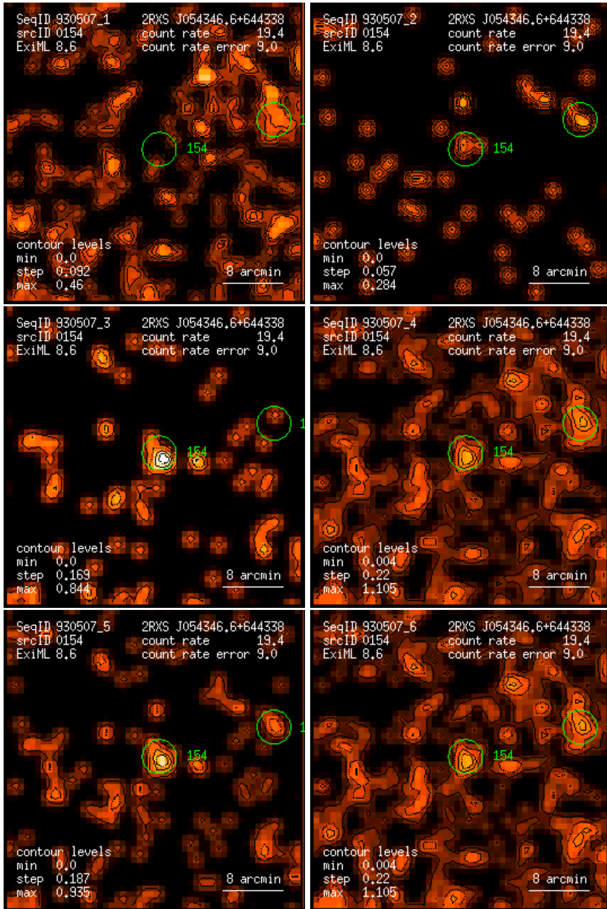
Figure 154: RASS 930507: detection 0154: band rate images, Gaussian filter: (1) PSPC channels 11 – 41, (2) 52 – 90, (3) 91 – 201, (4) 11 – 235, (5) 52 – 201, (6) 11 – 201. Broad band rates in counts/ks. Band rate contour levels in counts/ks/arcmin 2 .
