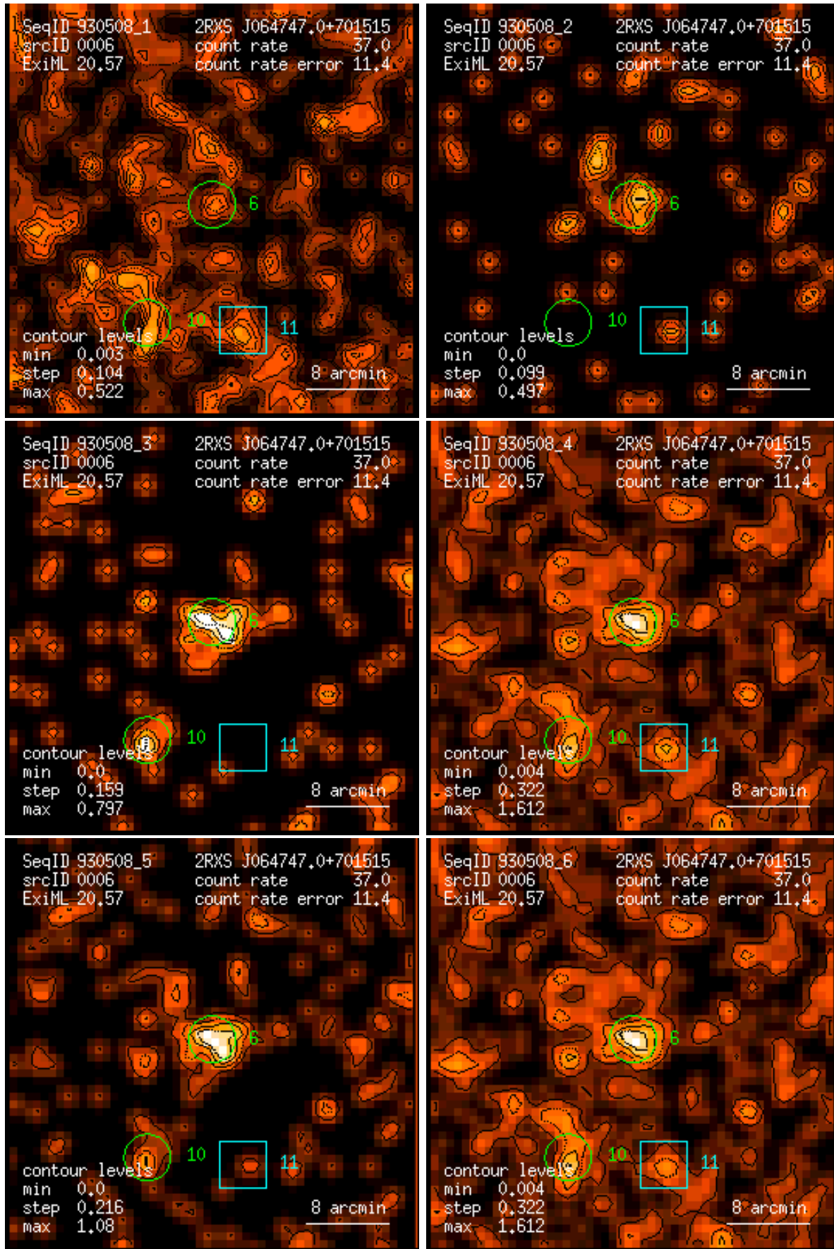
Figure 6: RASS 930508: detection 0006: band rate images, Gaussian filter: (1) PSPC channels 11 – 41, (2) 52 – 90, (3) 91 – 201, (4) 11 – 235, (5) 52 – 201, (6) 11 – 201. Broad band rates in counts/ks. Band rate contour levels in counts/ks/arcmin 2 .
