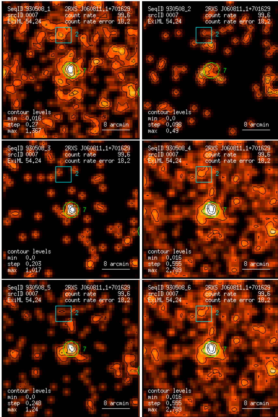
Figure 7: RASS 930508: detection 0007: band rate images, Gaussian filter: (1) PSPC channels 11 – 41, (2) 52 – 90, (3) 91 – 201, (4) 11 – 235, (5) 52 – 201, (6) 11 – 201. Broad band rates in counts/ks. Band rate contour levels in counts/ks/arcmin 2 .
