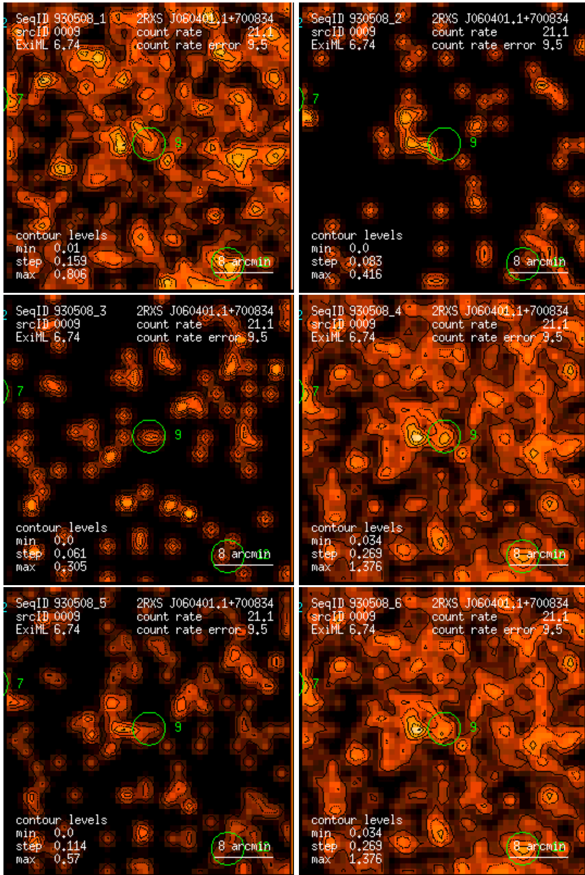
Figure 9: RASS 930508: detection 0009: band rate images, Gaussian filter: (1) PSPC channels 11 – 41, (2) 52 – 90, (3) 91 – 201, (4) 11 – 235, (5) 52 – 201, (6) 11 – 201. Broad band rates in counts/ks. Band rate contour levels in counts/ks/arcmin 2 .
