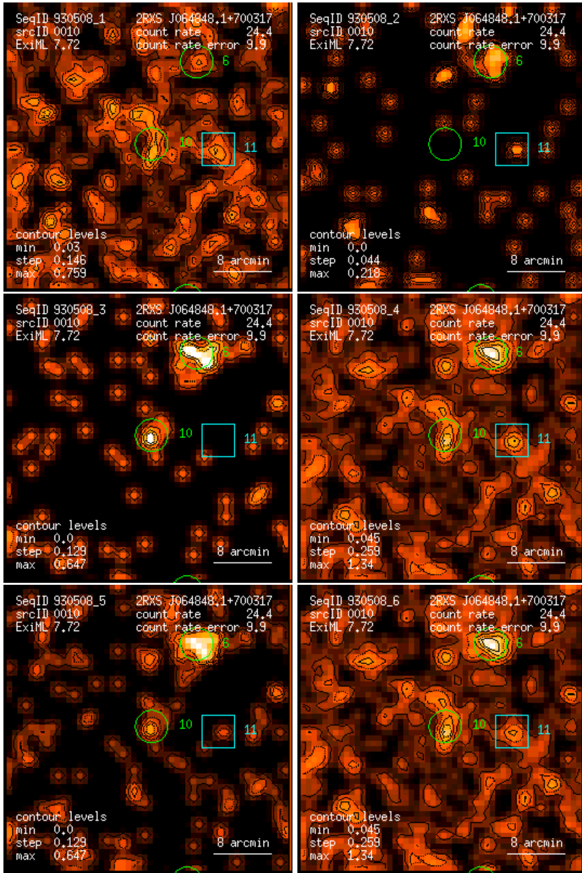
Figure 10: RASS 930508: detection 0010: band rate images, Gaussian filter: (1) PSPC channels 11 – 41, (2) 52 – 90, (3) 91 – 201, (4) 11 – 235, (5) 52 – 201, (6) 11 – 201. Broad band rates in counts/ks. Band rate contour levels in counts/ks/arcmin 2 .
