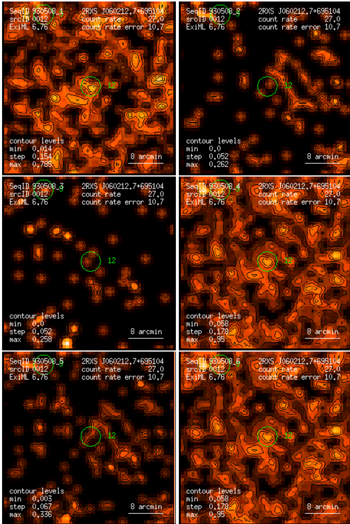
Figure 12: RASS 930508: detection 0012: band rate images, Gaussian filter: (1) PSPC channels 11 – 41, (2) 52 – 90, (3) 91 – 201, (4) 11 – 235, (5) 52 – 201, (6) 11 – 201. Broad band rates in counts/ks. Band rate contour levels in counts/ks/arcmin 2 .
