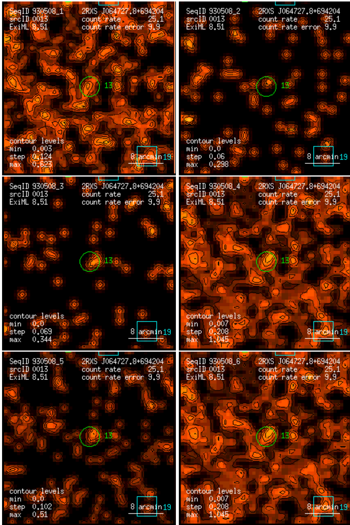
Figure 13: RASS 930508: detection 0013: band rate images, Gaussian filter: (1) PSPC channels 11 – 41, (2) 52 – 90, (3) 91 – 201, (4) 11 – 235, (5) 52 – 201, (6) 11 – 201. Broad band rates in counts/ks. Band rate contour levels in counts/ks/arcmin 2 .
