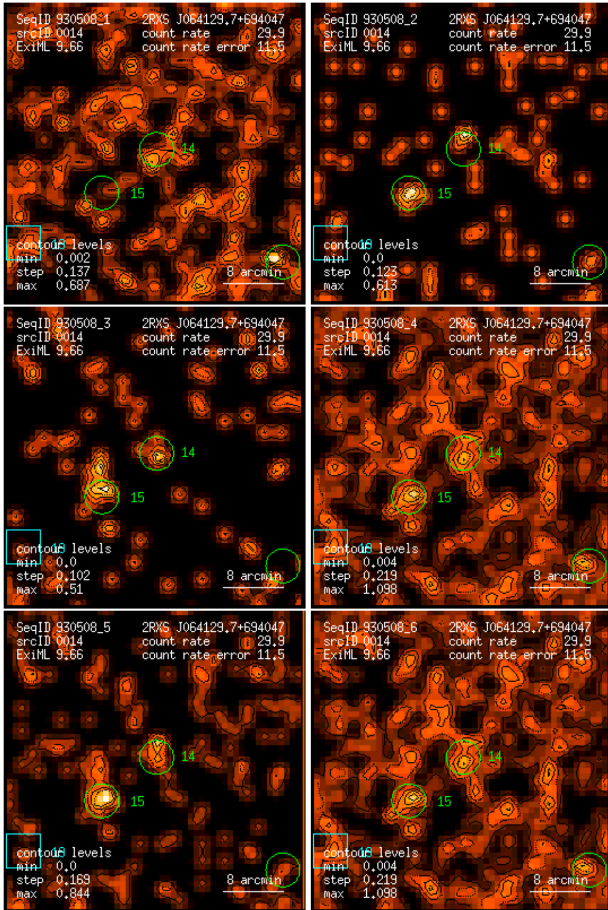
Figure 14: RASS 930508: detection 0014: band rate images, Gaussian filter: (1) PSPC channels 11 – 41, (2) 52 – 90, (3) 91 – 201, (4) 11 – 235, (5) 52 – 201, (6) 11 – 201. Broad band rates in counts/ks. Band rate contour levels in counts/ks/arcmin 2 .
