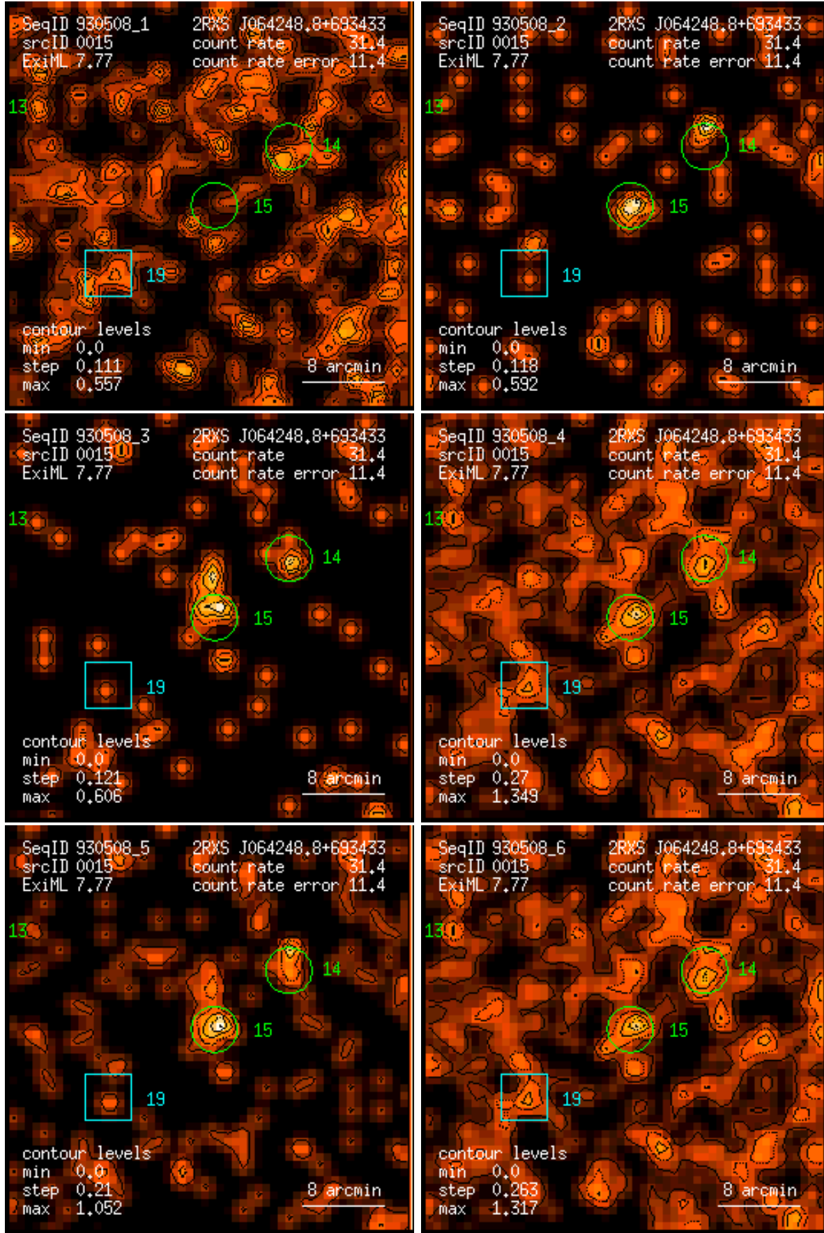
Figure 15: RASS 930508: detection 0015: band rate images, Gaussian filter: (1) PSPC channels 11 – 41, (2) 52 – 90, (3) 91 – 201, (4) 11 – 235, (5) 52 – 201, (6) 11 – 201. Broad band rates in counts/ks. Band rate contour levels in counts/ks/arcmin 2 .
