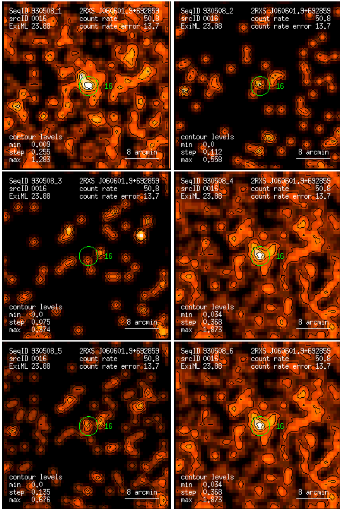
Figure 16: RASS 930508: detection 0016: band rate images, Gaussian filter: (1) PSPC channels 11 – 41, (2) 52 – 90, (3) 91 – 201, (4) 11 – 235, (5) 52 – 201, (6) 11 – 201. Broad band rates in counts/ks. Band rate contour levels in counts/ks/arcmin 2 .
