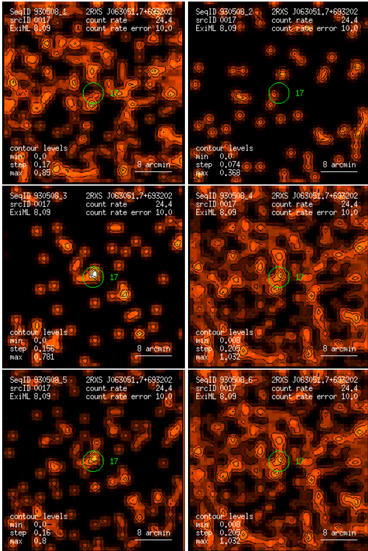
Figure 17: RASS 930508: detection 0017: band rate images, Gaussian filter: (1) PSPC channels 11 – 41, (2) 52 – 90, (3) 91 – 201, (4) 11 – 235, (5) 52 – 201, (6) 11 – 201. Broad band rates in counts/ks. Band rate contour levels in counts/ks/arcmin 2 .
