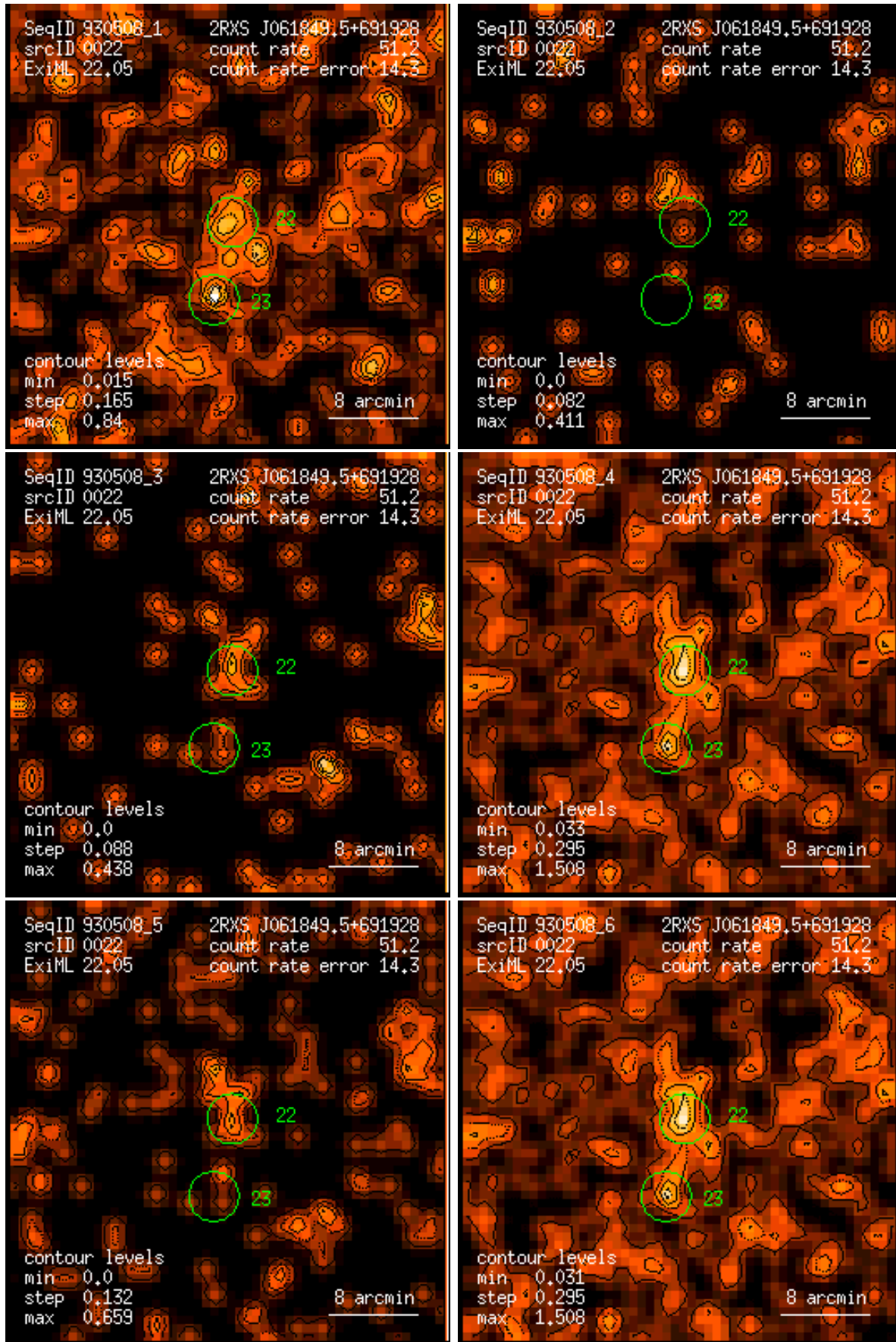
Figure 22: RASS 930508: detection 0022: band rate images, Gaussian filter: (1) PSPC channels 11 – 41, (2) 52 – 90, (3) 91 – 201, (4) 11 – 235, (5) 52 – 201, (6) 11 – 201. Broad band rates in counts/ks. Band rate contour levels in counts/ks/arcmin 2 .
