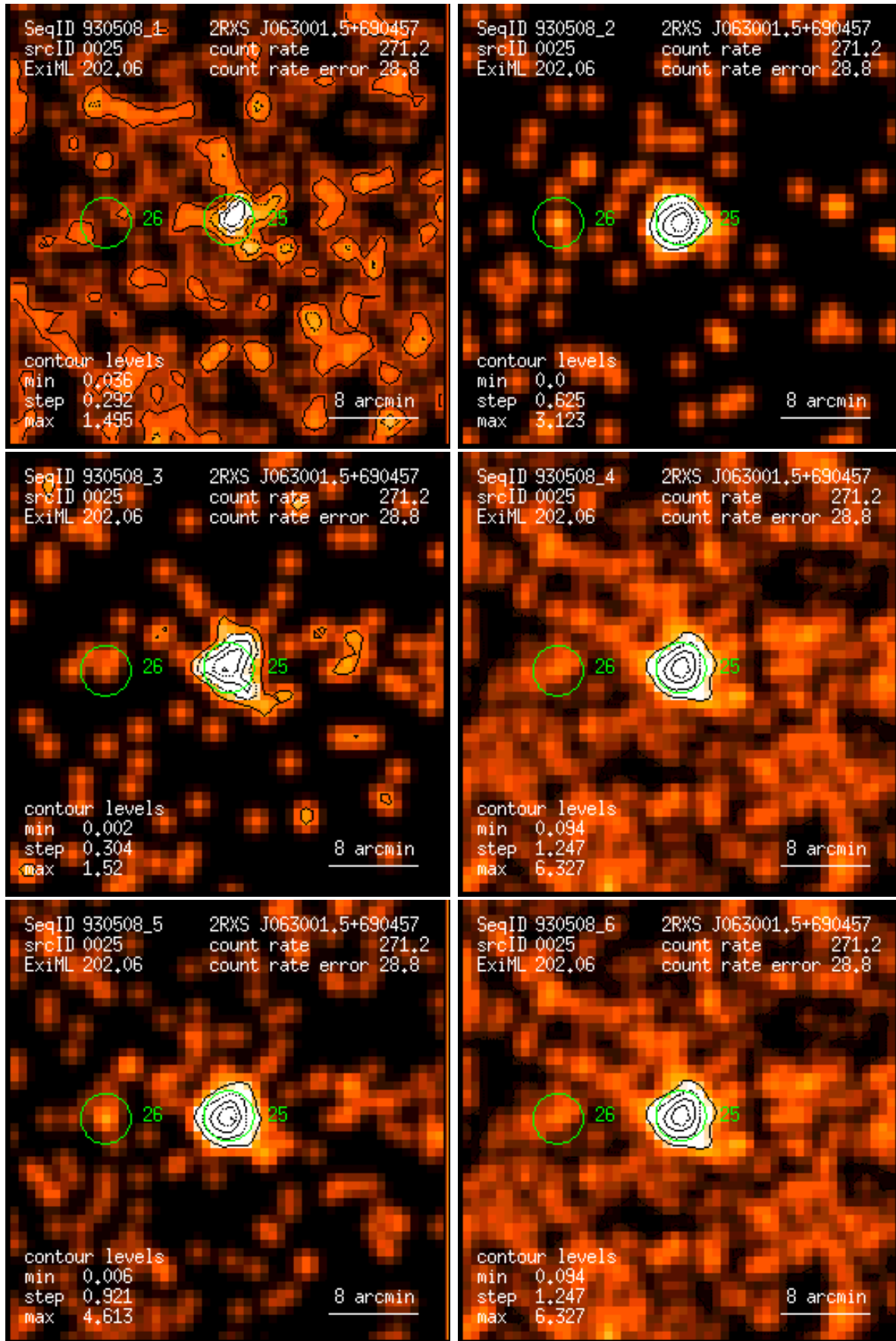
Figure 25: RASS 930508: detection 0025: band rate images, Gaussian filter: (1) PSPC channels 11 – 41, (2) 52 – 90, (3) 91 – 201, (4) 11 – 235, (5) 52 – 201, (6) 11 – 201. Broad band rates in counts/ks. Band rate contour levels in counts/ks/arcmin 2 .
