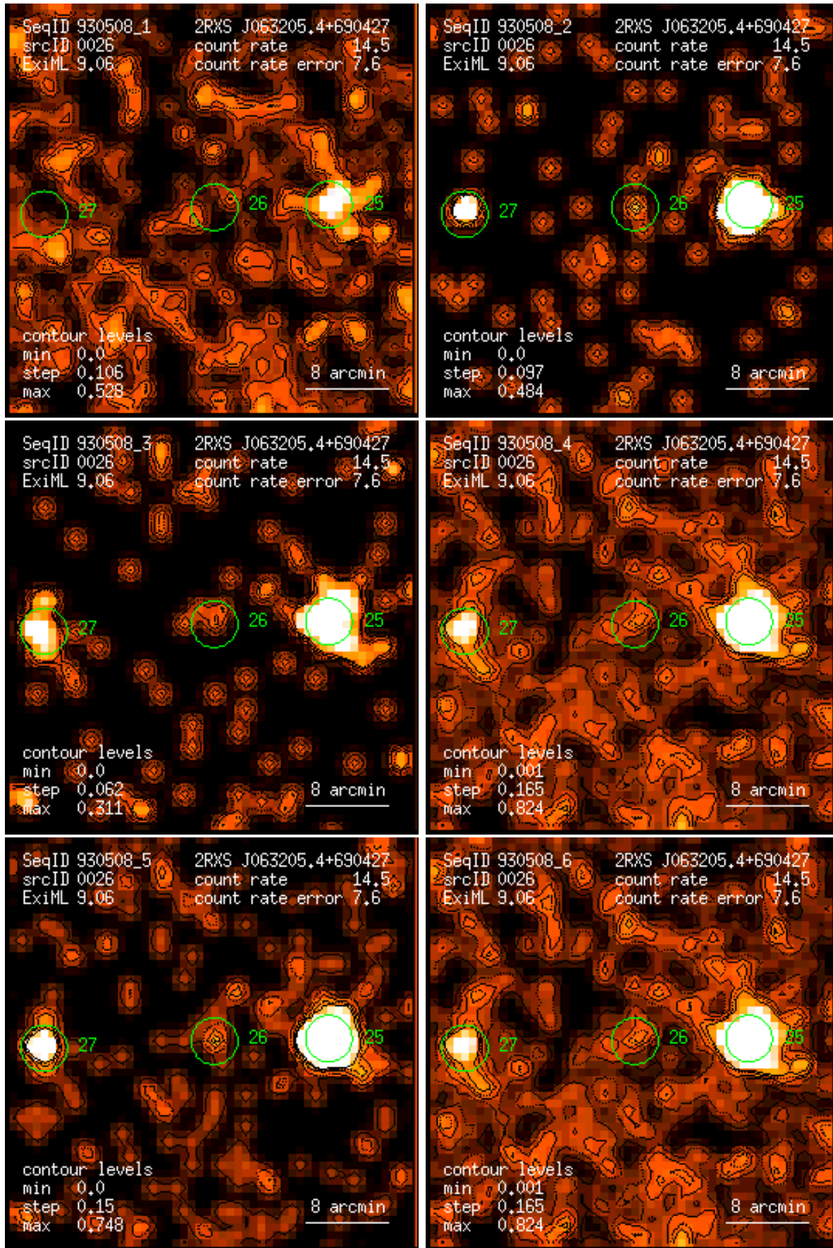
Figure 26: RASS 930508: detection 0026: band rate images, Gaussian filter: (1) PSPC channels 11 – 41, (2) 52 – 90, (3) 91 – 201, (4) 11 – 235, (5) 52 – 201, (6) 11 – 201. Broad band rates in counts/ks. Band rate contour levels in counts/ks/arcmin 2 .
