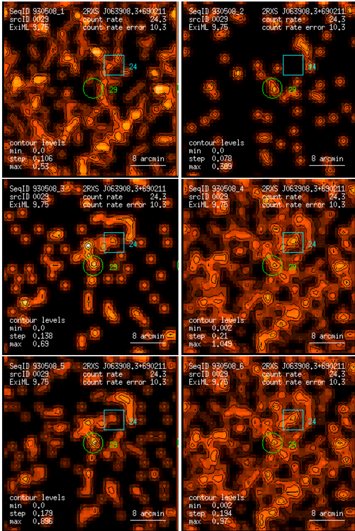
Figure 29: RASS 930508: detection 0029: band rate images, Gaussian filter: (1) PSPC channels 11 – 41, (2) 52 – 90, (3) 91 – 201, (4) 11 – 235, (5) 52 – 201, (6) 11 – 201. Broad band rates in counts/ks. Band rate contour levels in counts/ks/arcmin 2 .
