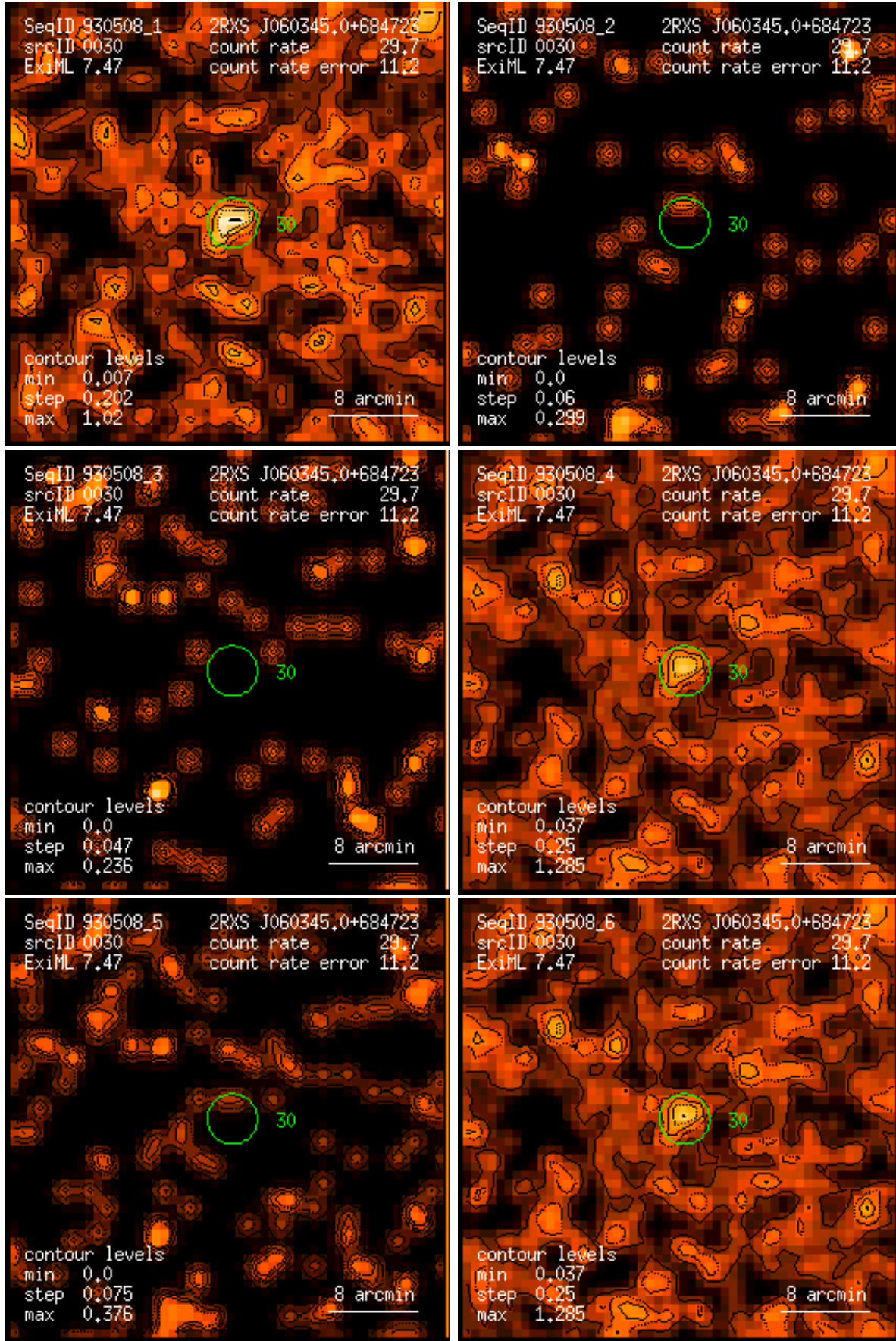
Figure 30: RASS 930508: detection 0030: band rate images, Gaussian filter: (1) PSPC channels 11 – 41, (2) 52 – 90, (3) 91 – 201, (4) 11 – 235, (5) 52 – 201, (6) 11 – 201. Broad band rates in counts/ks. Band rate contour levels in counts/ks/arcmin 2 .
