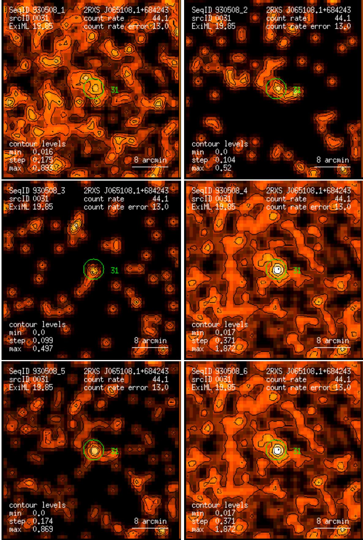
Figure 31: RASS 930508: detection 0031: band rate images, Gaussian filter: (1) PSPC channels 11 – 41, (2) 52 – 90, (3) 91 – 201, (4) 11 – 235, (5) 52 – 201, (6) 11 – 201. Broad band rates in counts/ks. Band rate contour levels in counts/ks/arcmin 2 .
