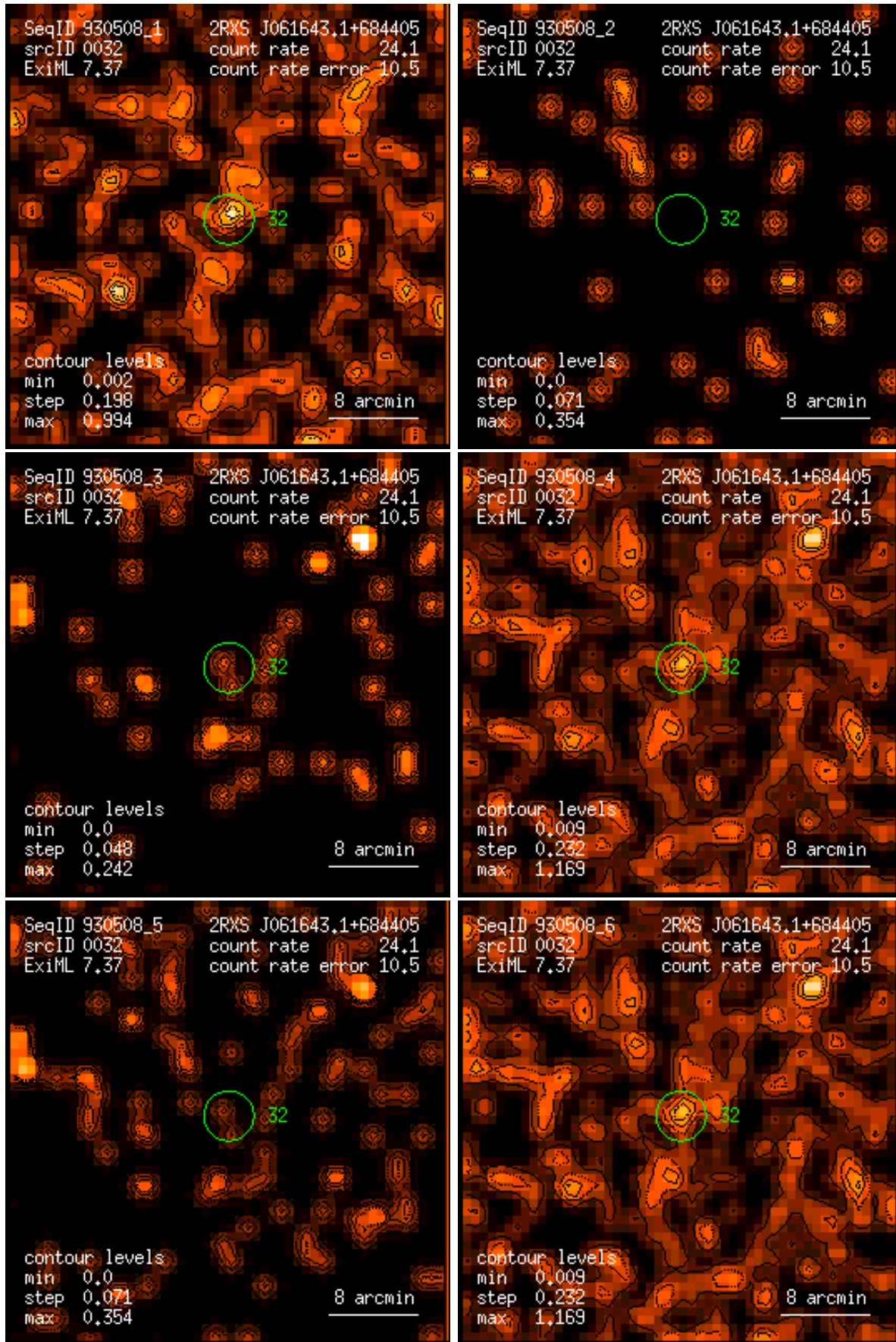
Figure 32: RASS 930508: detection 0032: band rate images, Gaussian filter: (1) PSPC channels 11 – 41, (2) 52 – 90, (3) 91 – 201, (4) 11 – 235, (5) 52 – 201, (6) 11 – 201. Broad band rates in counts/ks. Band rate contour levels in counts/ks/arcmin 2 .
