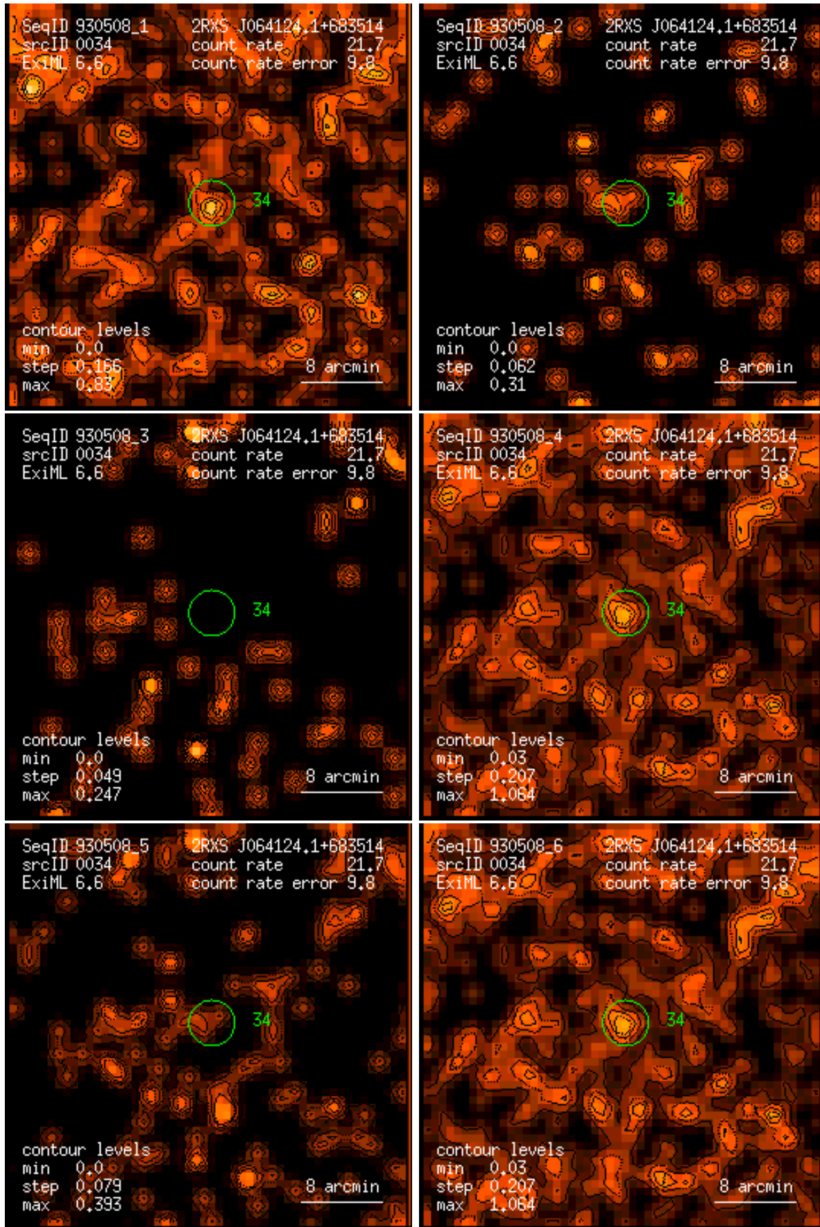
Figure 34: RASS 930508: detection 0034: band rate images, Gaussian filter: (1) PSPC channels 11 – 41, (2) 52 – 90, (3) 91 – 201, (4) 11 – 235, (5) 52 – 201, (6) 11 – 201. Broad band rates in counts/ks. Band rate contour levels in counts/ks/arcmin 2 .
