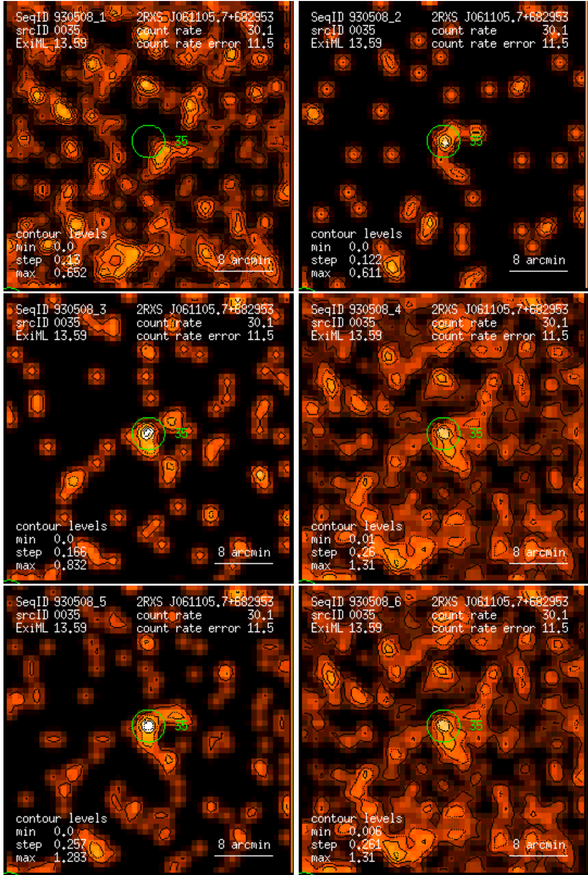
Figure 35: RASS 930508: detection 0035: band rate images, Gaussian filter: (1) PSPC channels 11 – 41, (2) 52 – 90, (3) 91 – 201, (4) 11 – 235, (5) 52 – 201, (6) 11 – 201. Broad band rates in counts/ks. Band rate contour levels in counts/ks/arcmin 2 .
