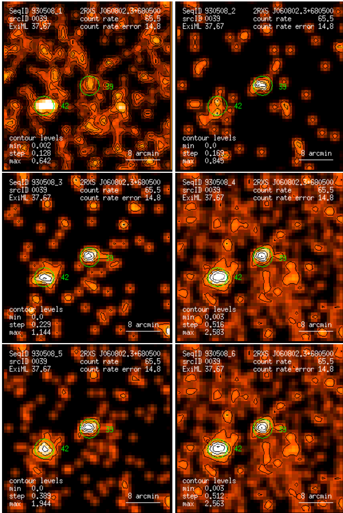
Figure 39: RASS 930508: detection 0039: band rate images, Gaussian filter: (1) PSPC channels 11 – 41, (2) 52 – 90, (3) 91 – 201, (4) 11 – 235, (5) 52 – 201, (6) 11 – 201. Broad band rates in counts/ks. Band rate contour levels in counts/ks/arcmin 2 .
