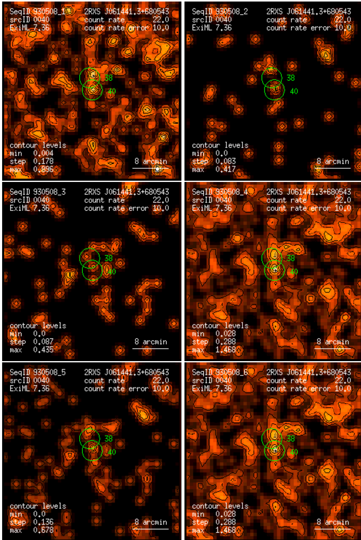
Figure 40: RASS 930508: detection 0040: band rate images, Gaussian filter: (1) PSPC channels 11 – 41, (2) 52 – 90, (3) 91 – 201, (4) 11 – 235, (5) 52 – 201, (6) 11 – 201. Broad band rates in counts/ks. Band rate contour levels in counts/ks/arcmin 2 .
