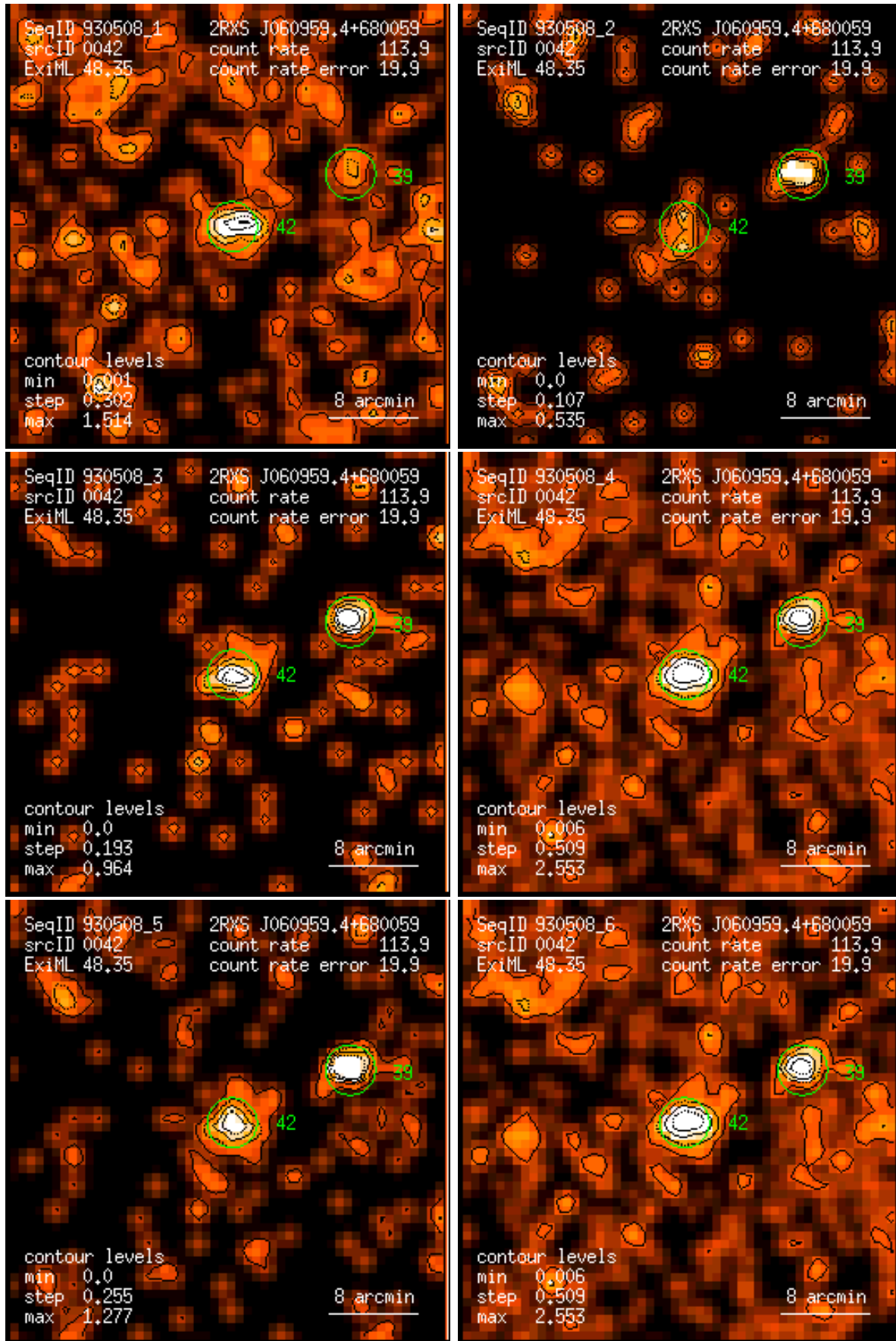
Figure 42: RASS 930508: detection 0042: band rate images, Gaussian filter: (1) PSPC channels 11 – 41, (2) 52 – 90, (3) 91 – 201, (4) 11 – 235, (5) 52 – 201, (6) 11 – 201. Broad band rates in counts/ks. Band rate contour levels in counts/ks/arcmin 2 .
