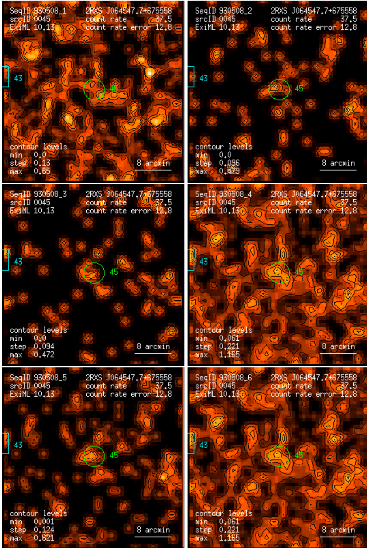
Figure 45: RASS 930508: detection 0045: band rate images, Gaussian filter: (1) PSPC channels 11 – 41, (2) 52 – 90, (3) 91 – 201, (4) 11 – 235, (5) 52 – 201, (6) 11 – 201. Broad band rates in counts/ks. Band rate contour levels in counts/ks/arcmin 2 .
