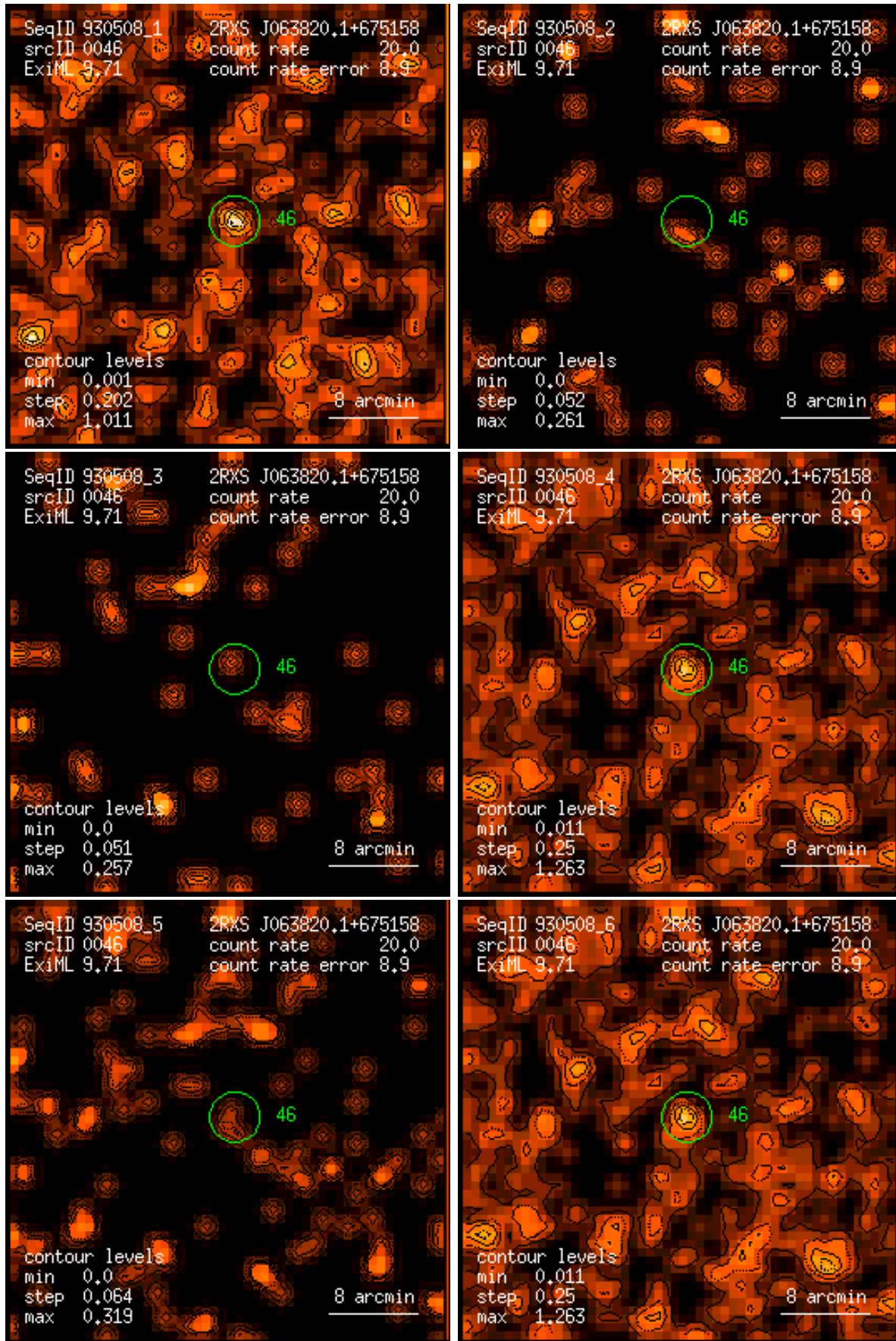
Figure 46: RASS 930508: detection 0046: band rate images, Gaussian filter: (1) PSPC channels 11 – 41, (2) 52 – 90, (3) 91 – 201, (4) 11 – 235, (5) 52 – 201, (6) 11 – 201. Broad band rates in counts/ks. Band rate contour levels in counts/ks/arcmin 2 .
