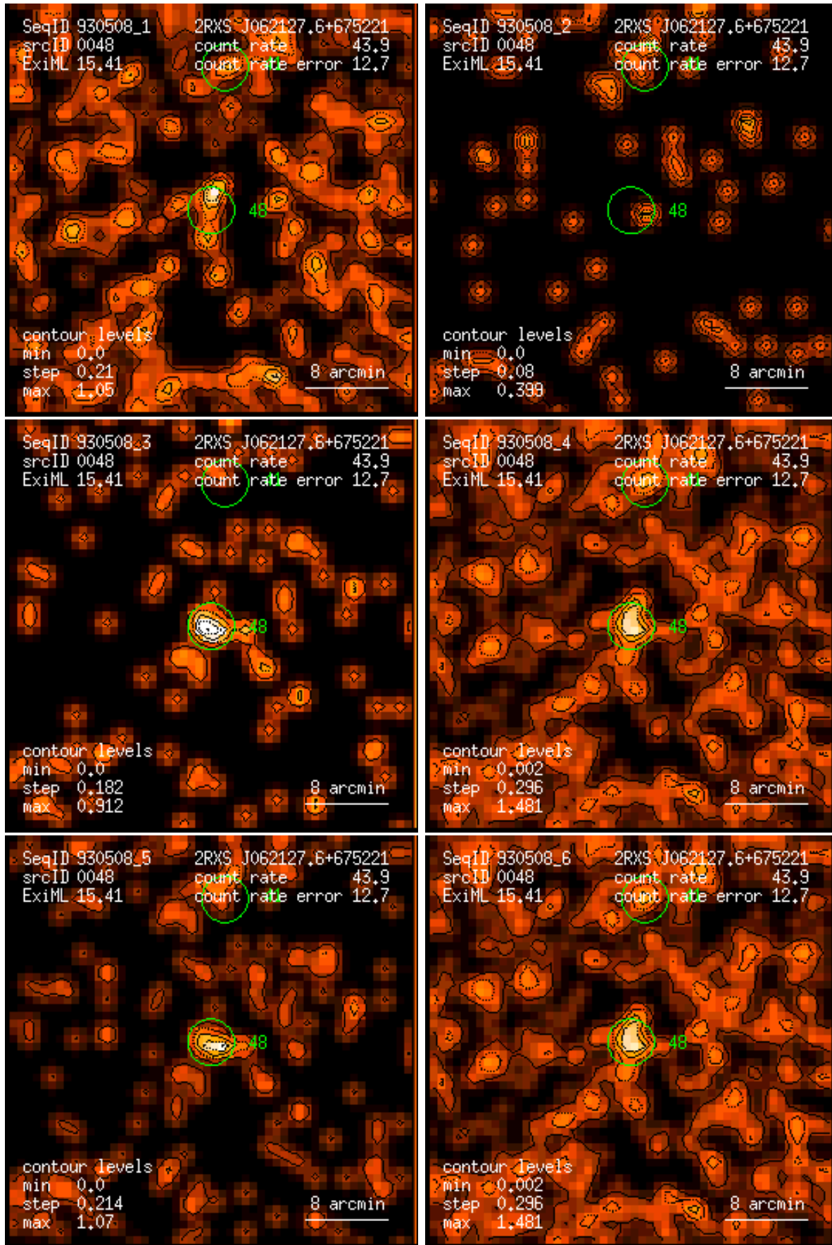
Figure 48: RASS 930508: detection 0048: band rate images, Gaussian filter: (1) PSPC channels 11 – 41, (2) 52 – 90, (3) 91 – 201, (4) 11 – 235, (5) 52 – 201, (6) 11 – 201. Broad band rates in counts/ks. Band rate contour levels in counts/ks/arcmin 2 .
