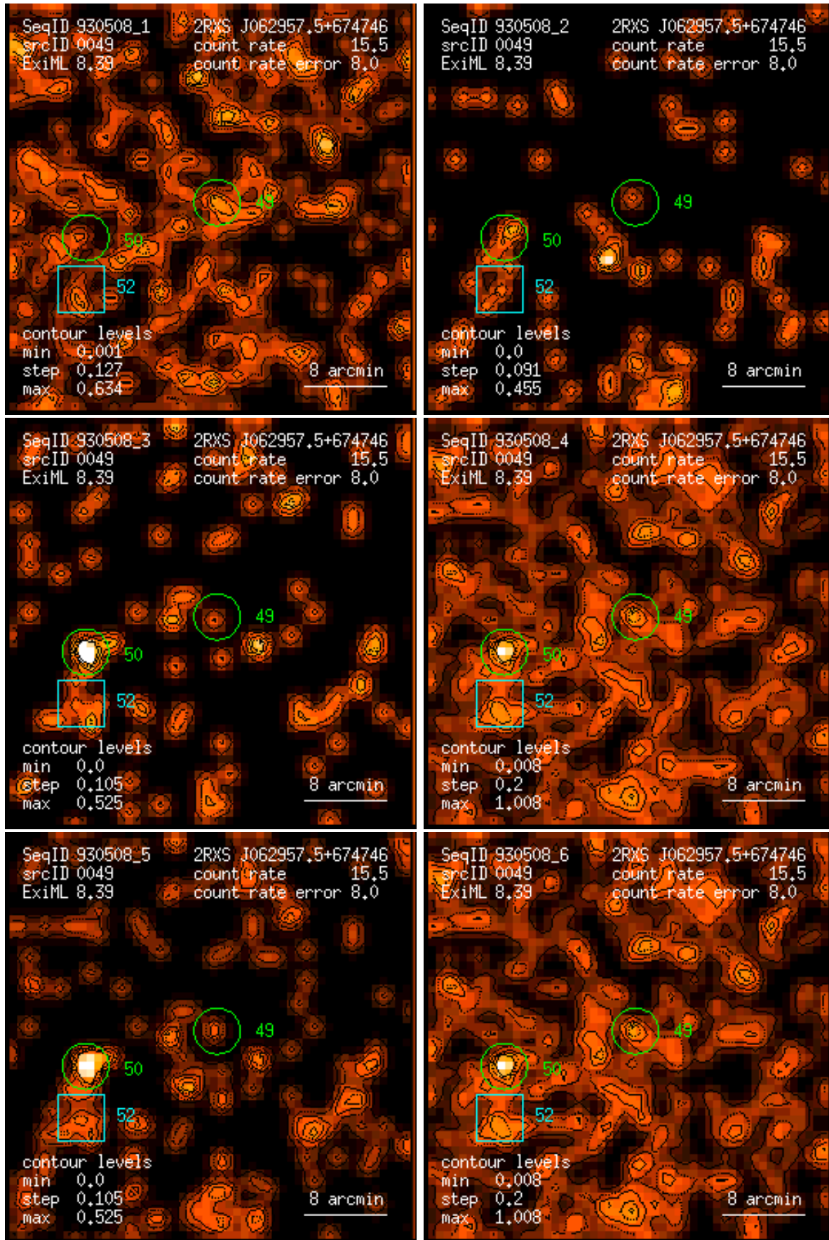
Figure 49: RASS 930508: detection 0049: band rate images, Gaussian filter: (1) PSPC channels 11 – 41, (2) 52 – 90, (3) 91 – 201, (4) 11 – 235, (5) 52 – 201, (6) 11 – 201. Broad band rates in counts/ks. Band rate contour levels in counts/ks/arcmin 2 .
