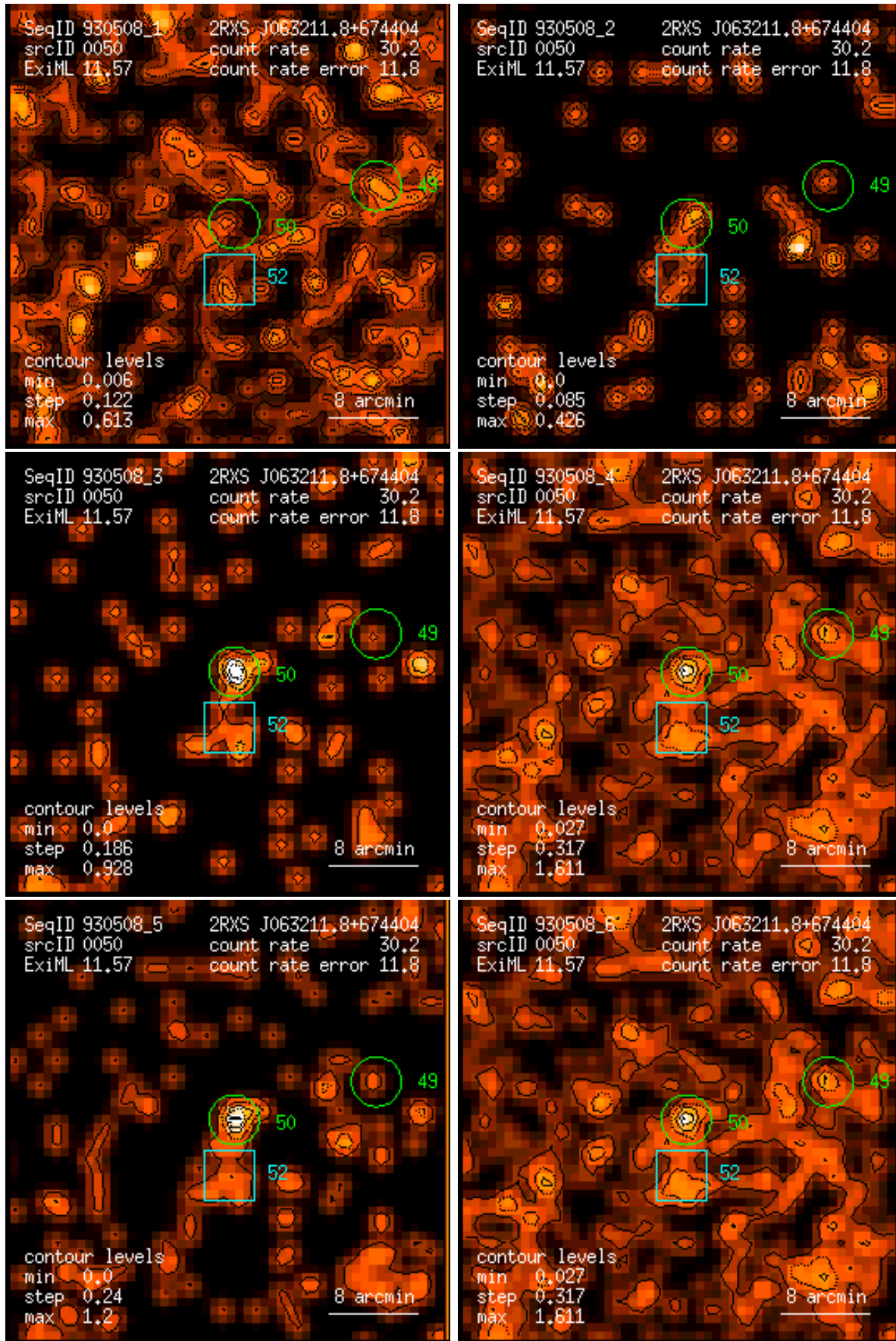
Figure 50: RASS 930508: detection 0050: band rate images, Gaussian filter: (1) PSPC channels 11 – 41, (2) 52 – 90, (3) 91 – 201, (4) 11 – 235, (5) 52 – 201, (6) 11 – 201. Broad band rates in counts/ks. Band rate contour levels in counts/ks/arcmin 2 .
