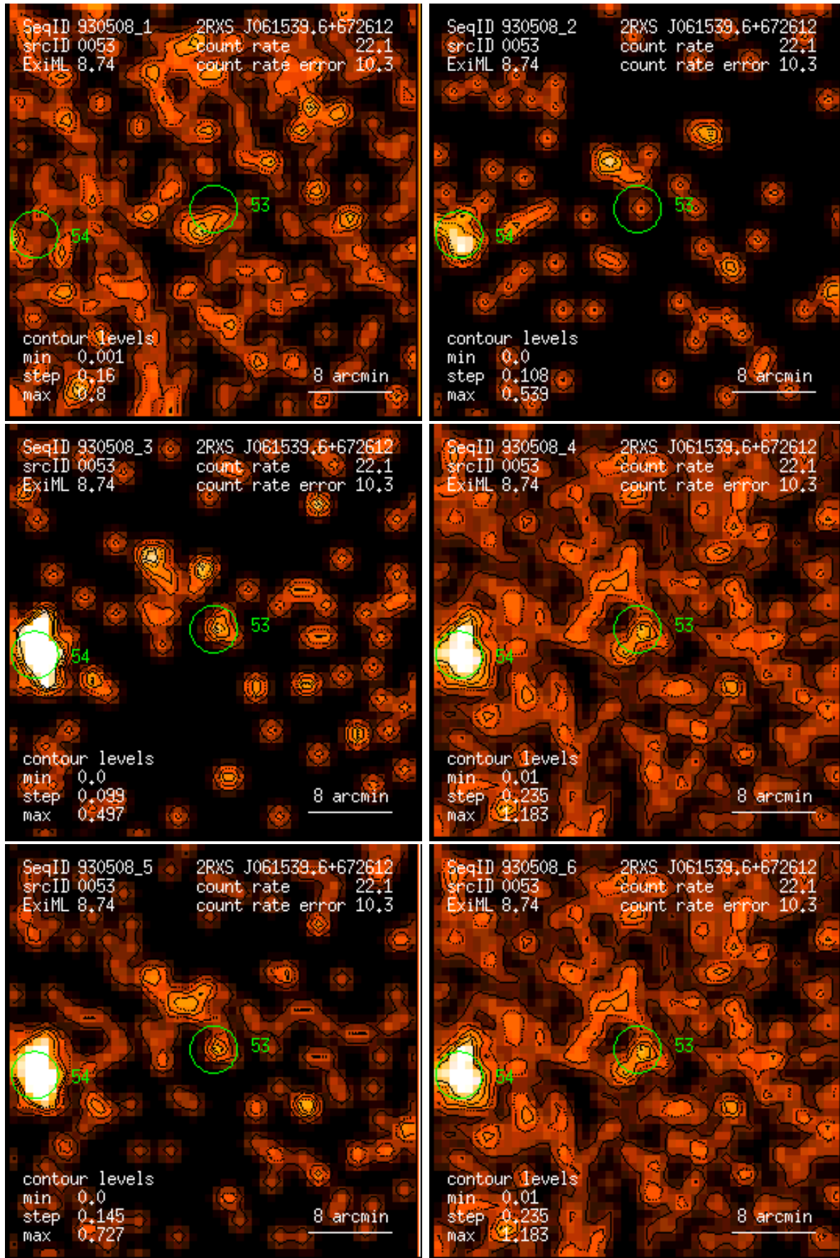
Figure 53: RASS 930508: detection 0053: band rate images, Gaussian filter: (1) PSPC channels 11 – 41, (2) 52 – 90, (3) 91 – 201, (4) 11 – 235, (5) 52 – 201, (6) 11 – 201. Broad band rates in counts/ks. Band rate contour levels in counts/ks/arcmin 2 .
