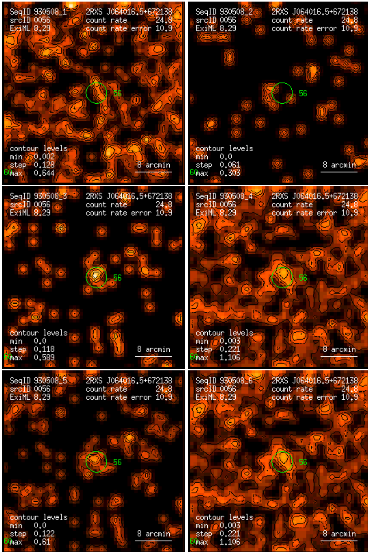
Figure 56: RASS 930508: detection 0056: band rate images, Gaussian filter: (1) PSPC channels 11 – 41, (2) 52 – 90, (3) 91 – 201, (4) 11 – 235, (5) 52 – 201, (6) 11 – 201. Broad band rates in counts/ks. Band rate contour levels in counts/ks/arcmin 2 .
