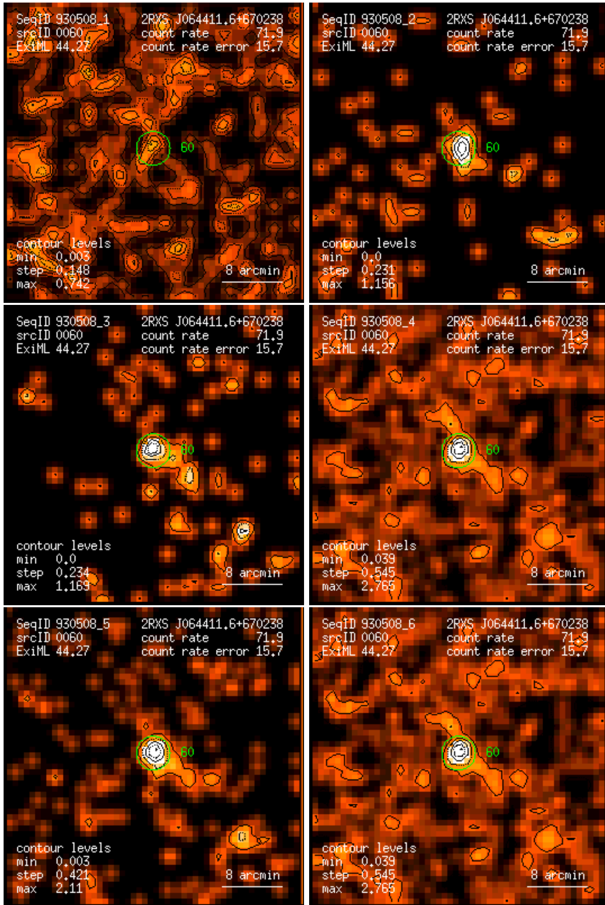
Figure 60: RASS 930508: detection 0060: band rate images, Gaussian filter: (1) PSPC channels 11 – 41, (2) 52 – 90, (3) 91 – 201, (4) 11 – 235, (5) 52 – 201, (6) 11 – 201. Broad band rates in counts/ks. Band rate contour levels in counts/ks/arcmin 2 .
