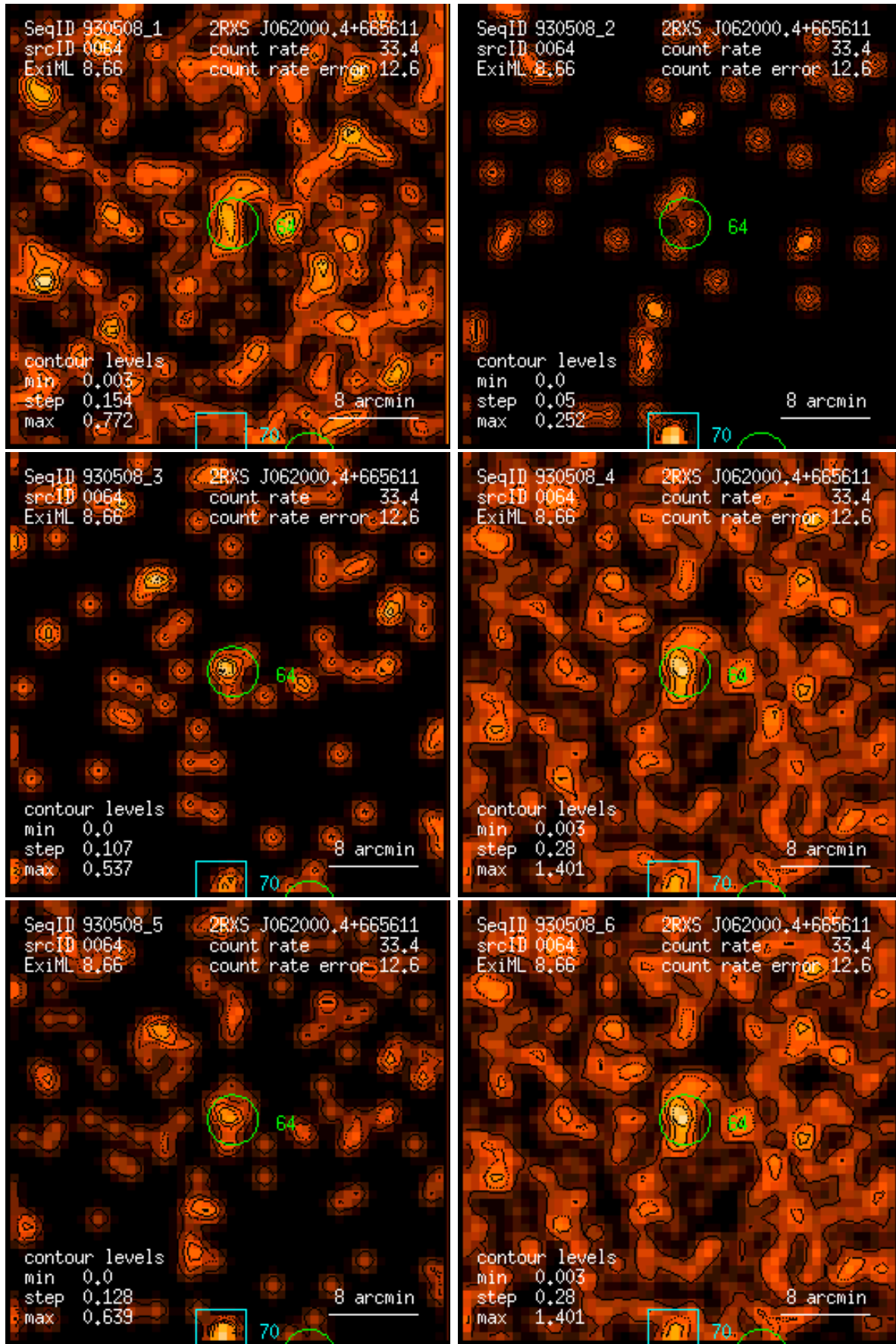
Figure 64: RASS 930508: detection 0064: band rate images, Gaussian filter: (1) PSPC channels 11 – 41, (2) 52 – 90, (3) 91 – 201, (4) 11 – 235, (5) 52 – 201, (6) 11 – 201. Broad band rates in counts/ks. Band rate contour levels in counts/ks/arcmin 2 .
