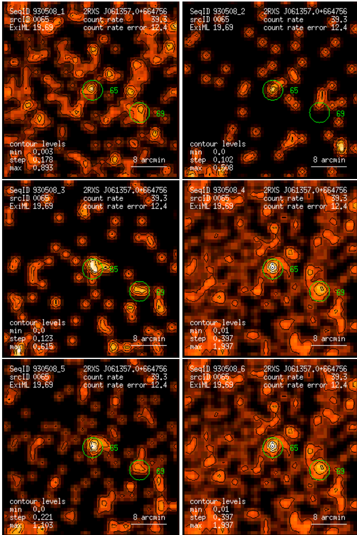
Figure 65: RASS 930508: detection 0065: band rate images, Gaussian filter: (1) PSPC channels 11 – 41, (2) 52 – 90, (3) 91 – 201, (4) 11 – 235, (5) 52 – 201, (6) 11 – 201. Broad band rates in counts/ks. Band rate contour levels in counts/ks/arcmin 2 .
