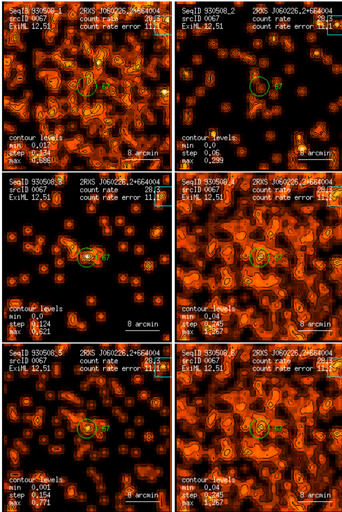
Figure 67: RASS 930508: detection 0067: band rate images, Gaussian filter: (1) PSPC channels 11 – 41, (2) 52 – 90, (3) 91 – 201, (4) 11 – 235, (5) 52 – 201, (6) 11 – 201. Broad band rates in counts/ks. Band rate contour levels in counts/ks/arcmin 2 .
