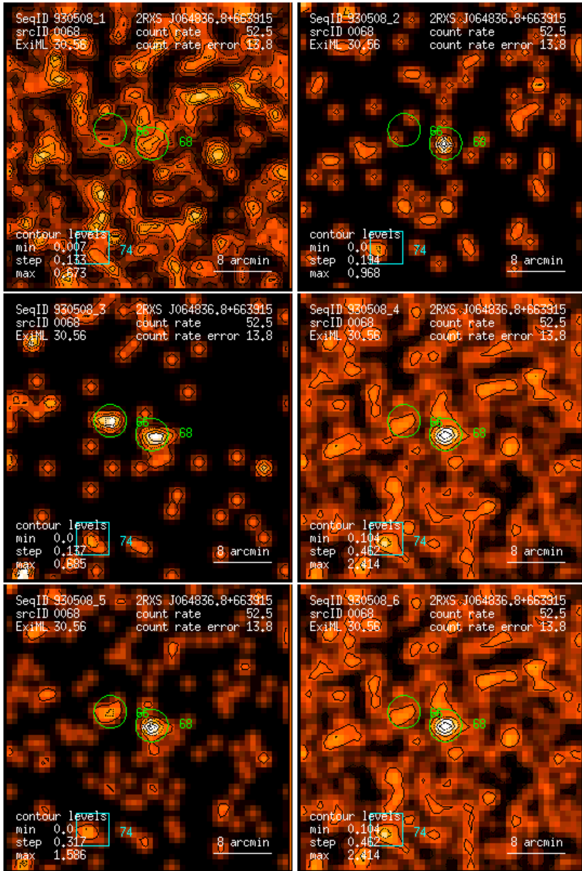
Figure 68: RASS 930508: detection 0068: band rate images, Gaussian filter: (1) PSPC channels 11 – 41, (2) 52 – 90, (3) 91 – 201, (4) 11 – 235, (5) 52 – 201, (6) 11 – 201. Broad band rates in counts/ks. Band rate contour levels in counts/ks/arcmin 2 .
