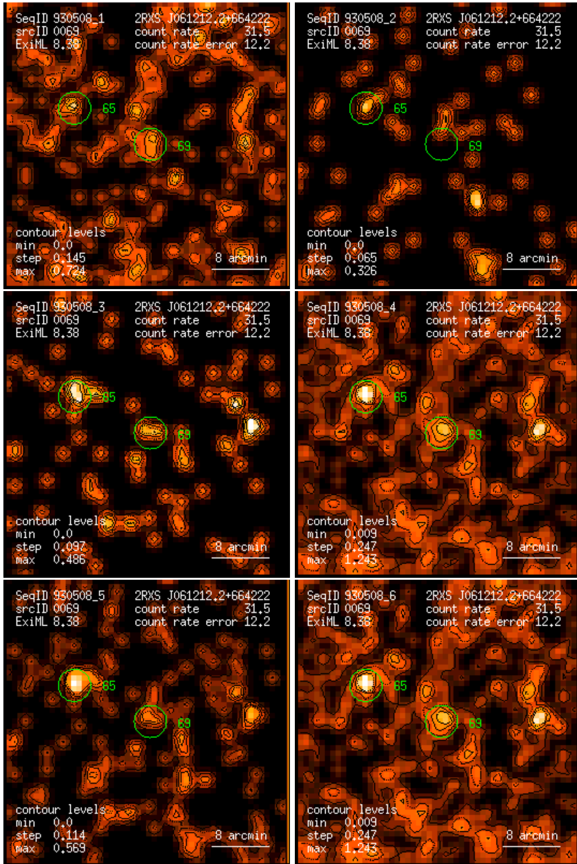
Figure 69: RASS 930508: detection 0069: band rate images, Gaussian filter: (1) PSPC channels 11 – 41, (2) 52 – 90, (3) 91 – 201, (4) 11 – 235, (5) 52 – 201, (6) 11 – 201. Broad band rates in counts/ks. Band rate contour levels in counts/ks/arcmin 2 .
