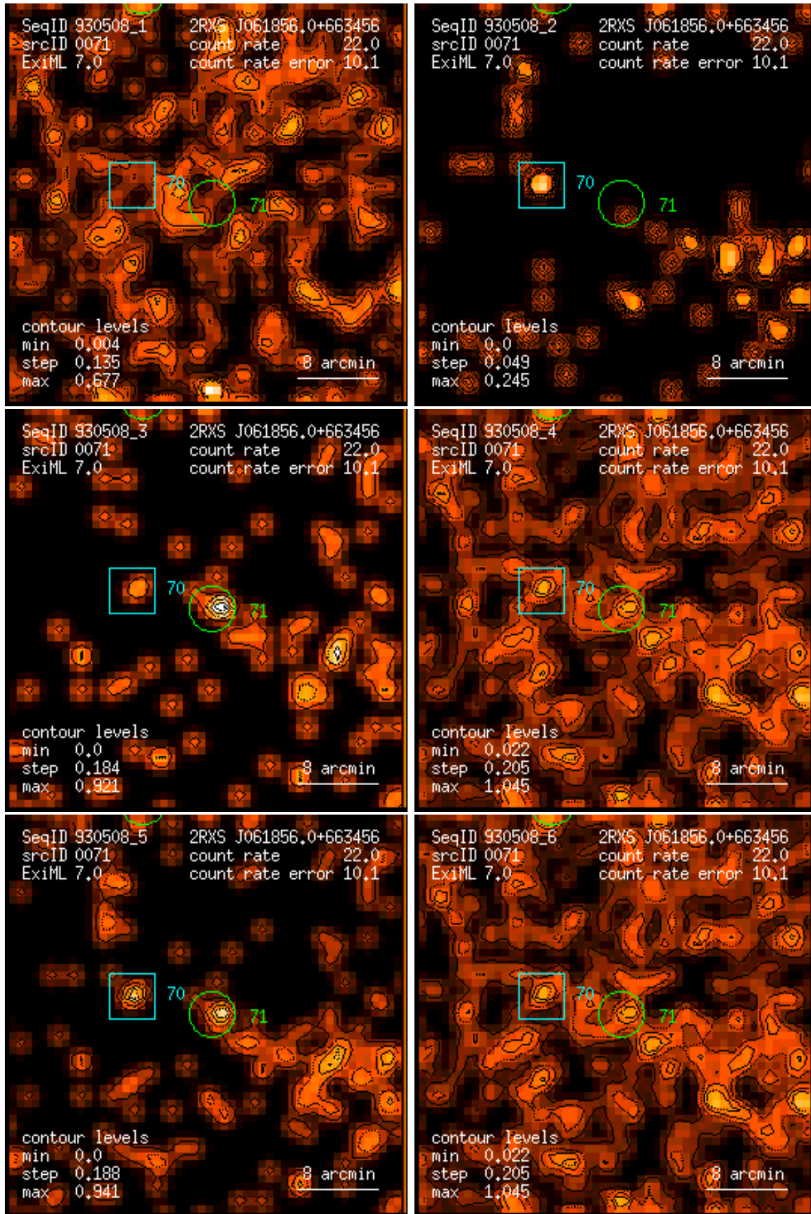
Figure 71: RASS 930508: detection 0071: band rate images, Gaussian filter: (1) PSPC channels 11 – 41, (2) 52 – 90, (3) 91 – 201, (4) 11 – 235, (5) 52 – 201, (6) 11 – 201. Broad band rates in counts/ks. Band rate contour levels in counts/ks/arcmin 2 .
