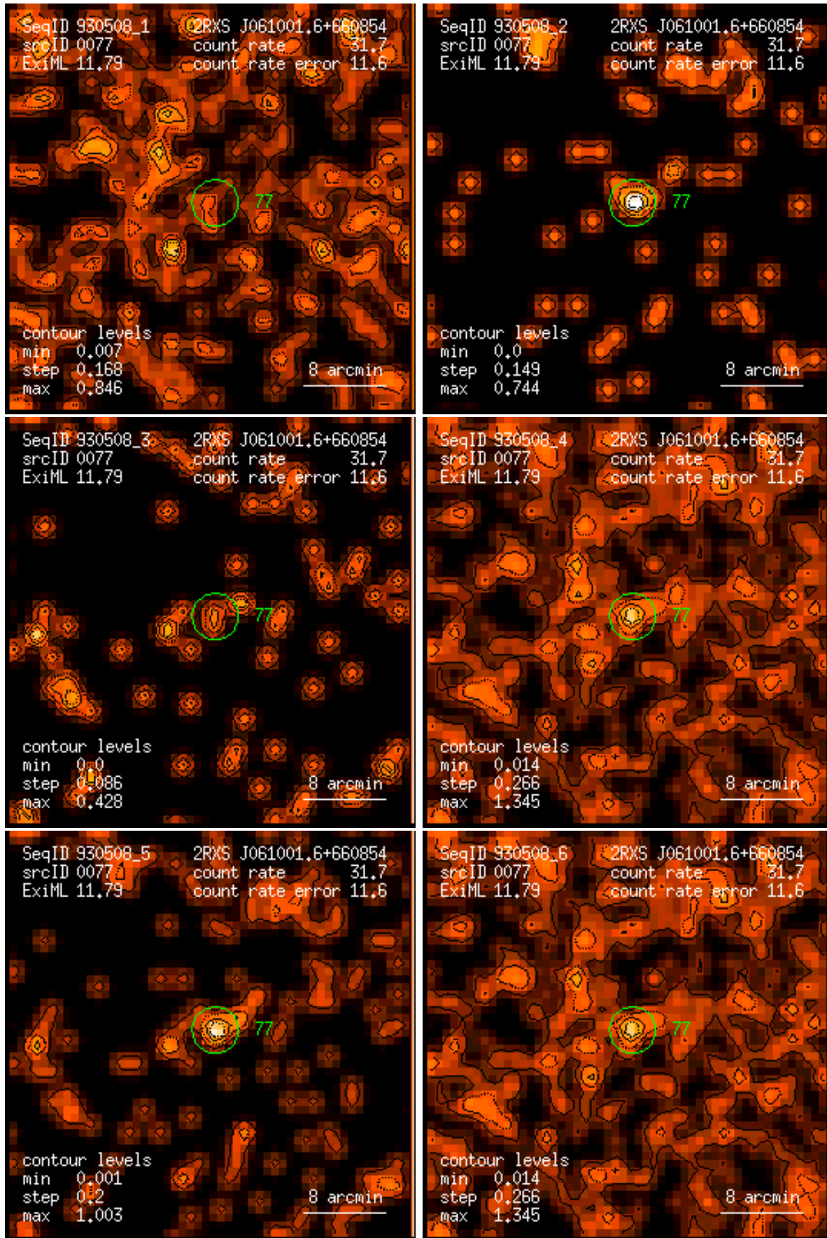
Figure 77: RASS 930508: detection 0077: band rate images, Gaussian filter: (1) PSPC channels 11 – 41, (2) 52 – 90, (3) 91 – 201, (4) 11 – 235, (5) 52 – 201, (6) 11 – 201. Broad band rates in counts/ks. Band rate contour levels in counts/ks/arcmin 2 .
