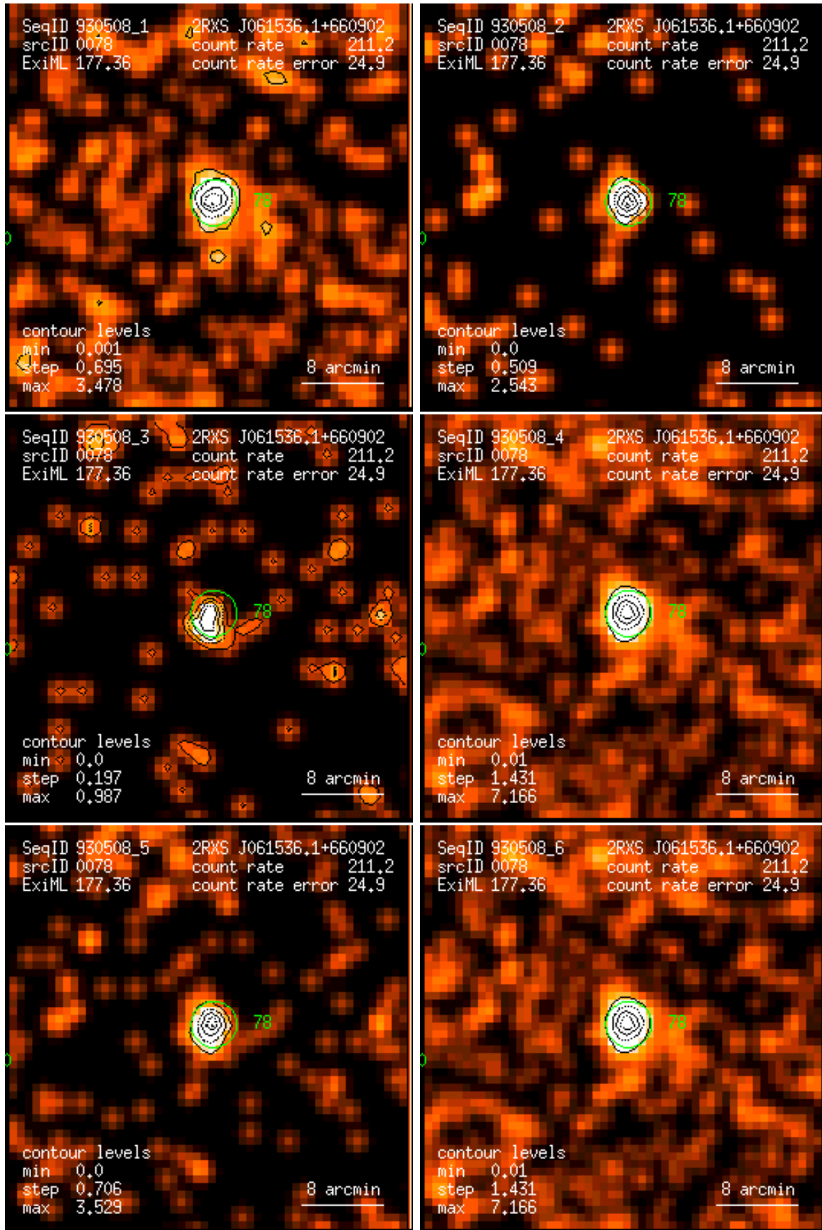
Figure 78: RASS 930508: detection 0078: band rate images, Gaussian filter: (1) PSPC channels 11 – 41, (2) 52 – 90, (3) 91 – 201, (4) 11 – 235, (5) 52 – 201, (6) 11 – 201. Broad band rates in counts/ks. Band rate contour levels in counts/ks/arcmin 2 .
