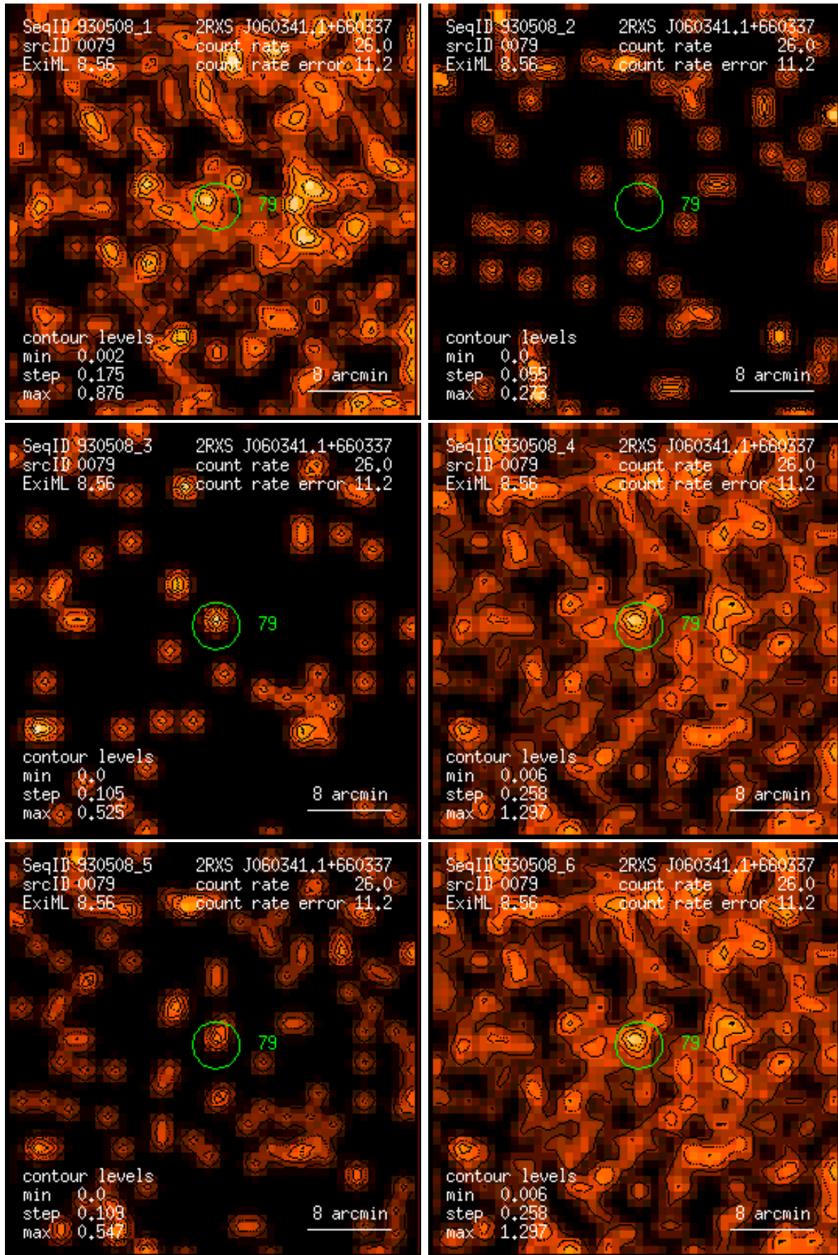
Figure 79: RASS 930508: detection 0079: band rate images, Gaussian filter: (1) PSPC channels 11 – 41, (2) 52 – 90, (3) 91 – 201, (4) 11 – 235, (5) 52 – 201, (6) 11 – 201. Broad band rates in counts/ks. Band rate contour levels in counts/ks/arcmin 2 .
