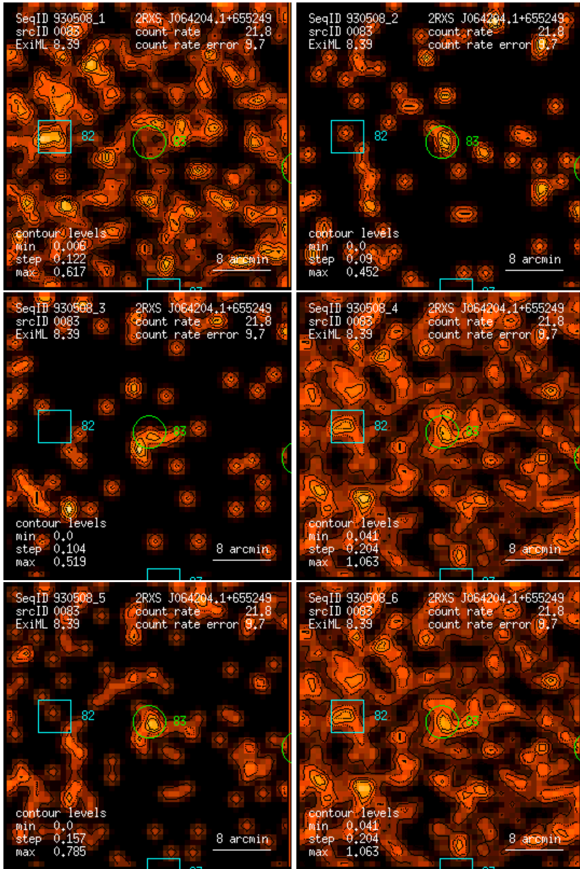
Figure 83: RASS 930508: detection 0083: band rate images, Gaussian filter: (1) PSPC channels 11 – 41, (2) 52 – 90, (3) 91 – 201, (4) 11 – 235, (5) 52 – 201, (6) 11 – 201. Broad band rates in counts/ks. Band rate contour levels in counts/ks/arcmin 2 .
