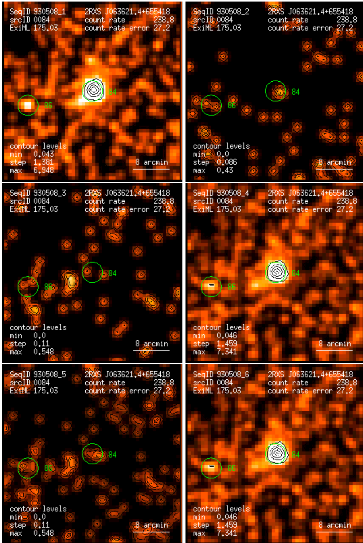
Figure 84: RASS 930508: detection 0084: band rate images, Gaussian filter: (1) PSPC channels 11 – 41, (2) 52 – 90, (3) 91 – 201, (4) 11 – 235, (5) 52 – 201, (6) 11 – 201. Broad band rates in counts/ks. Band rate contour levels in counts/ks/arcmin 2 .
