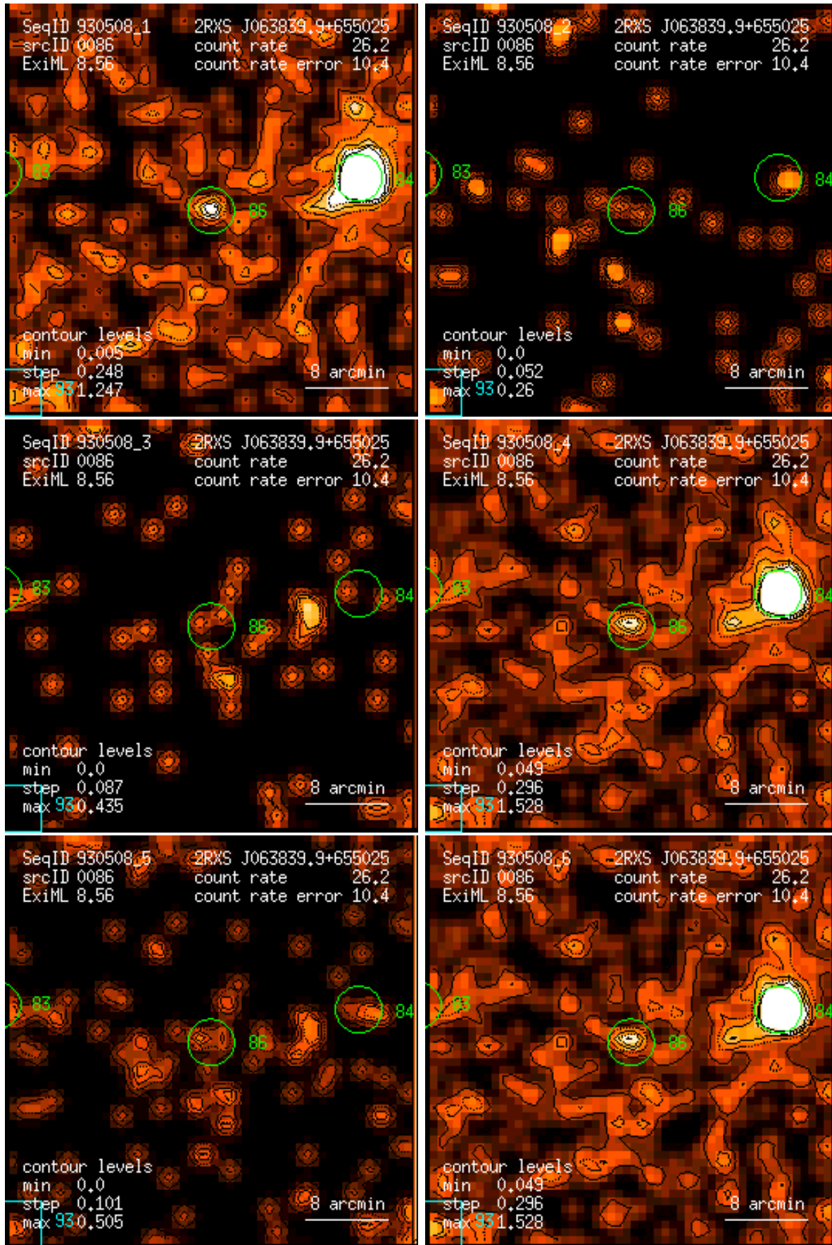
Figure 86: RASS 930508: detection 0086: band rate images, Gaussian filter: (1) PSPC channels 11 – 41, (2) 52 – 90, (3) 91 – 201, (4) 11 – 235, (5) 52 – 201, (6) 11 – 201. Broad band rates in counts/ks. Band rate contour levels in counts/ks/arcmin 2 .
