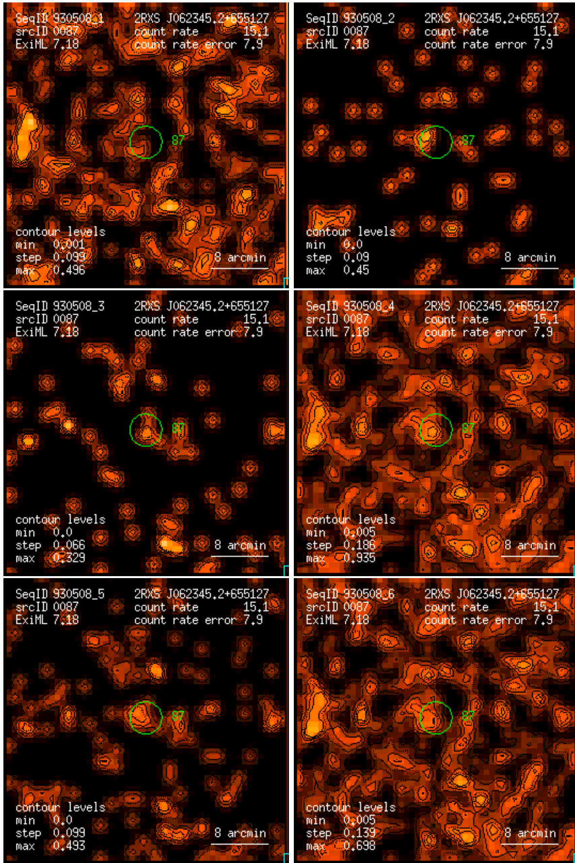
Figure 87: RASS 930508: detection 0087: band rate images, Gaussian filter: (1) PSPC channels 11 – 41, (2) 52 – 90, (3) 91 – 201, (4) 11 – 235, (5) 52 – 201, (6) 11 – 201. Broad band rates in counts/ks. Band rate contour levels in counts/ks/arcmin 2 .
