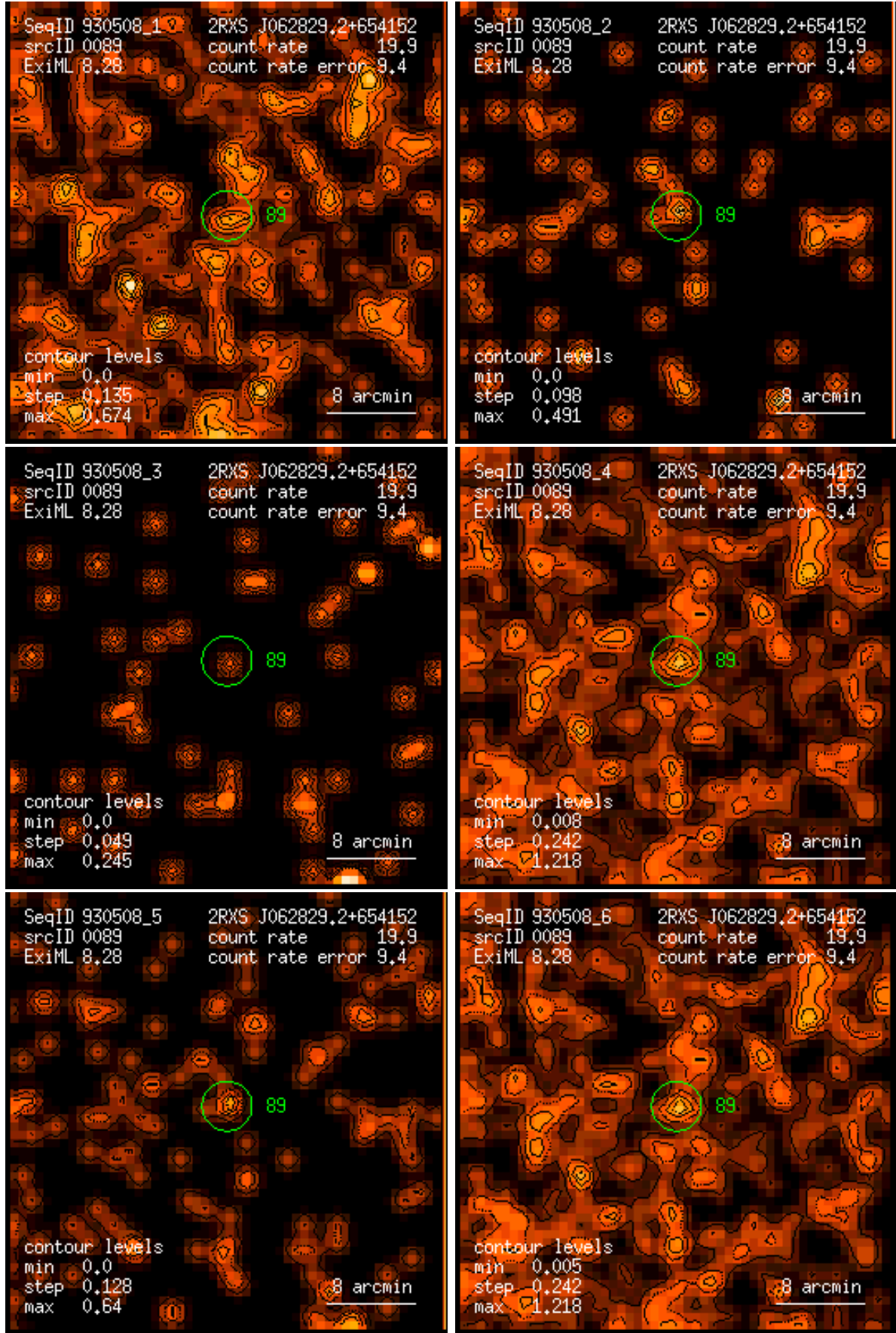
Figure 89: RASS 930508: detection 0089: band rate images, Gaussian filter: (1) PSPC channels 11 – 41, (2) 52 – 90, (3) 91 – 201, (4) 11 – 235, (5) 52 – 201, (6) 11 – 201. Broad band rates in counts/ks. Band rate contour levels in counts/ks/arcmin 2 .
