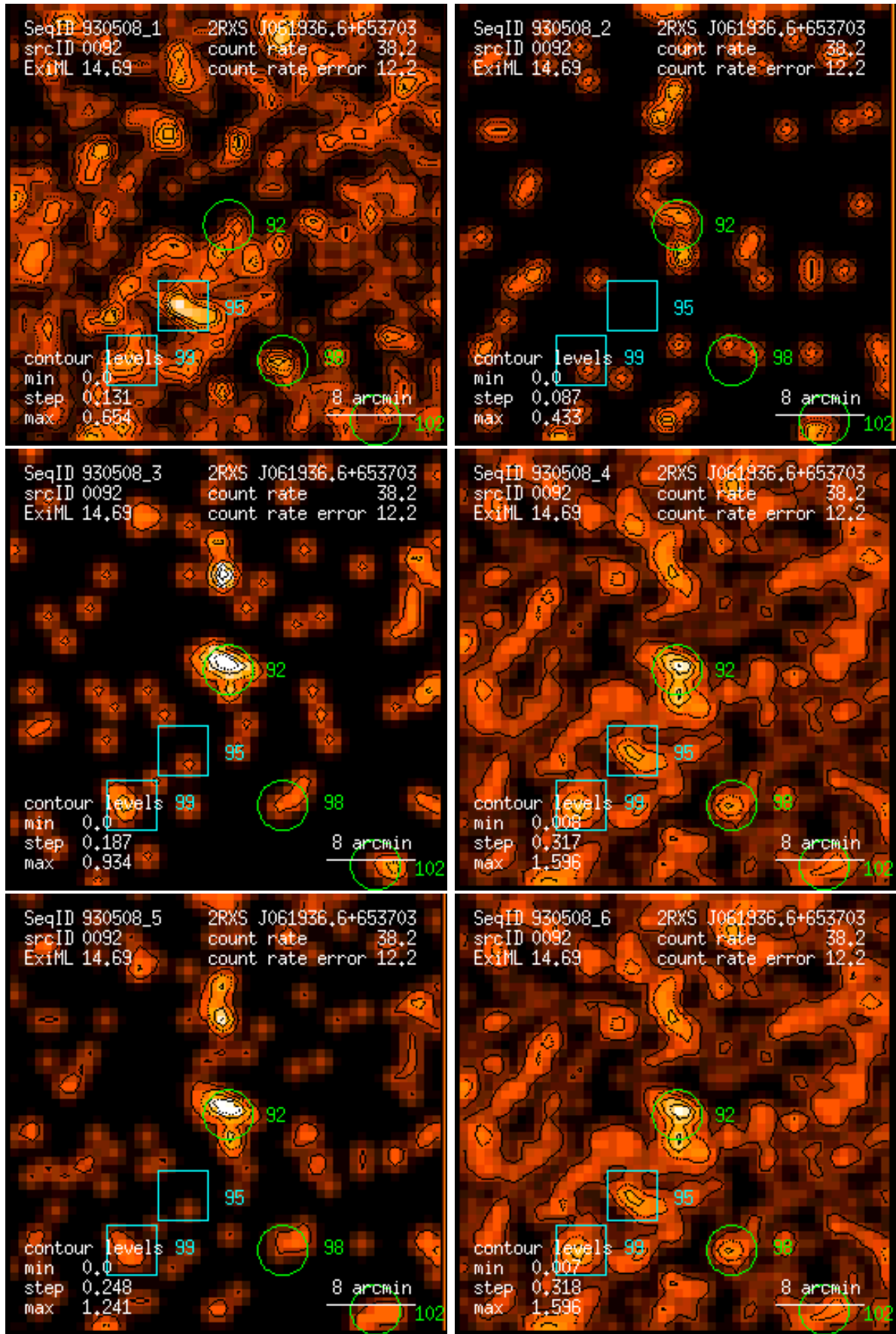
Figure 92: RASS 930508: detection 0092: band rate images, Gaussian filter: (1) PSPC channels 11 – 41, (2) 52 – 90, (3) 91 – 201, (4) 11 – 235, (5) 52 – 201, (6) 11 – 201. Broad band rates in counts/ks. Band rate contour levels in counts/ks/arcmin 2 .
