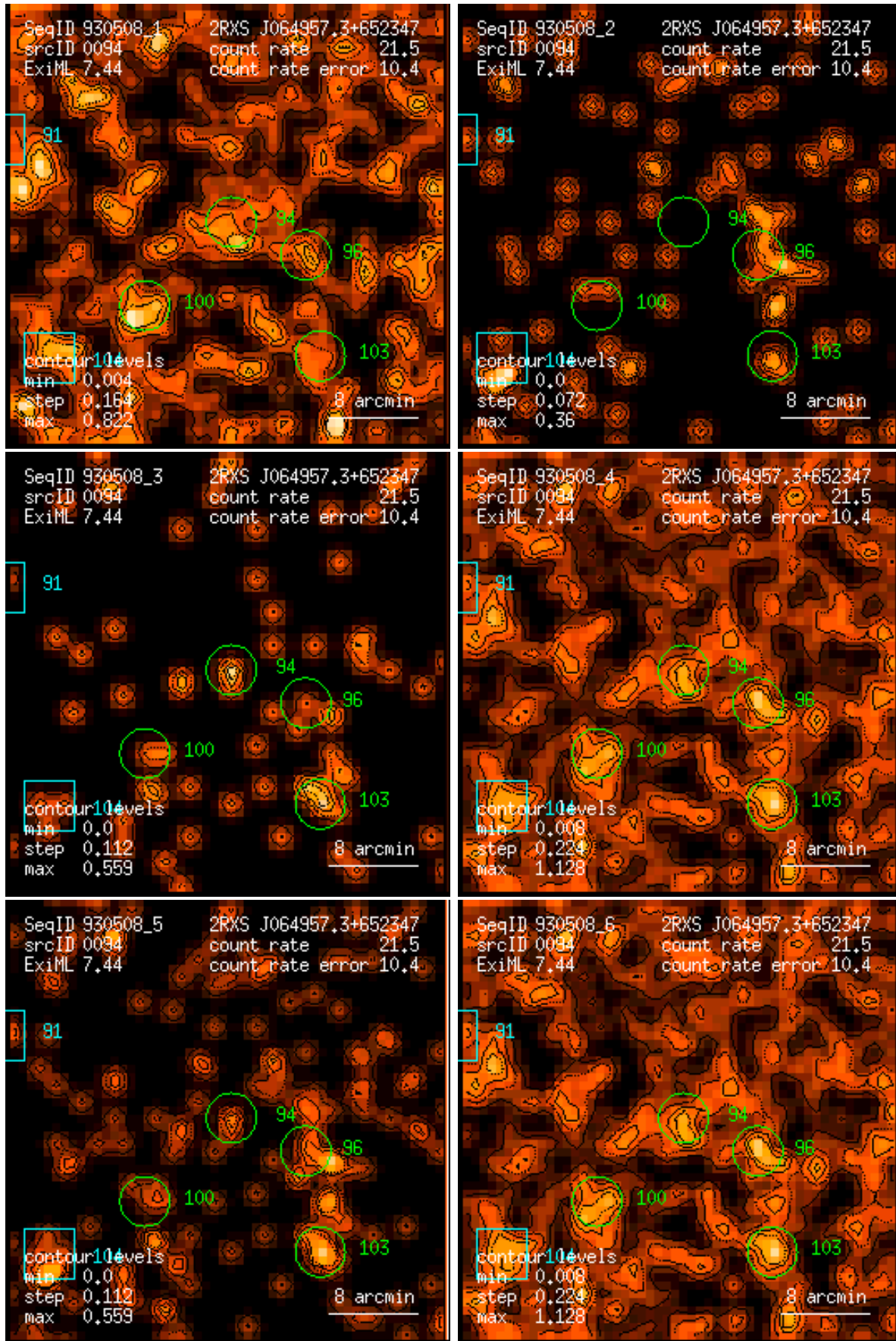
Figure 94: RASS 930508: detection 0094: band rate images, Gaussian filter: (1) PSPC channels 11 – 41, (2) 52 – 90, (3) 91 – 201, (4) 11 – 235, (5) 52 – 201, (6) 11 – 201. Broad band rates in counts/ks. Band rate contour levels in counts/ks/arcmin 2 .
